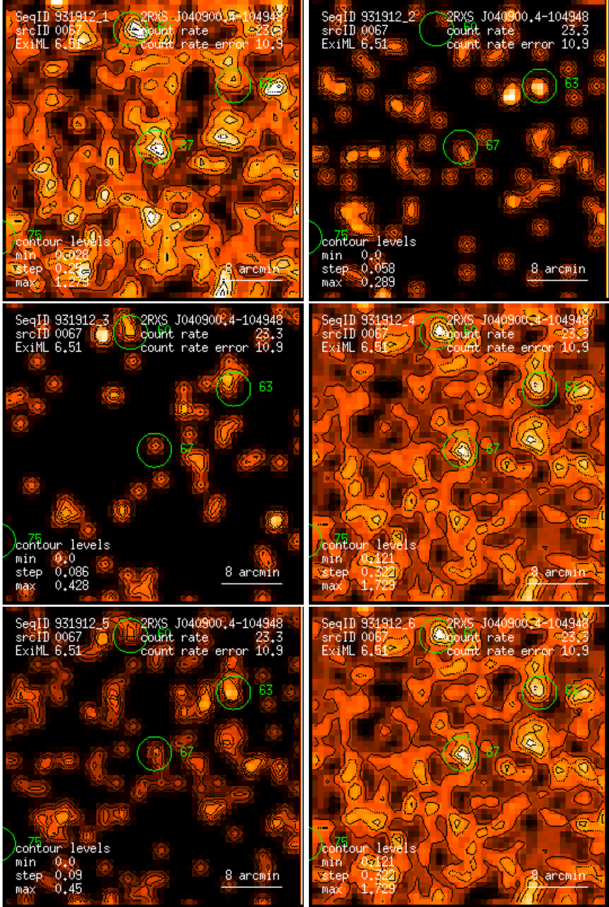
Figure 67: RASS 931912: detection 0067: band rate images, Gaussian filter: (1) PSPC channels 11 – 41, (2) 52 – 90, (3) 91 – 201, (4) 11 – 235, (5) 52 – 201, (6) 11 – 201. Broad band rates in counts/ks. Band rate contour levels in counts/ks/arcmin 2 .
