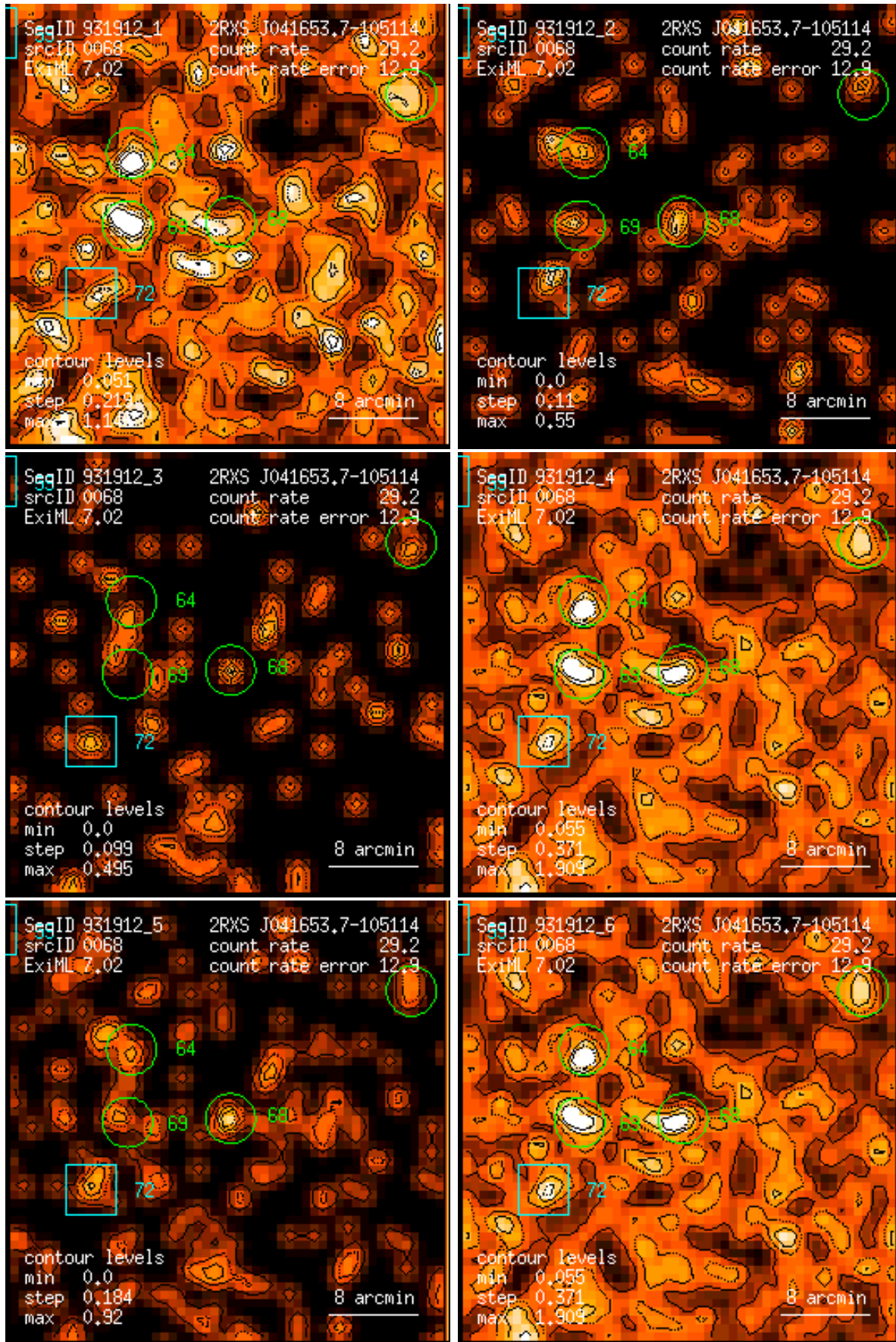
Figure 68: RASS 931912: detection 0068: band rate images, Gaussian filter: (1) PSPC channels 11 – 41, (2) 52 – 90, (3) 91 – 201, (4) 11 – 235, (5) 52 – 201, (6) 11 – 201. Broad band rates in counts/ks. Band rate contour levels in counts/ks/arcmin 2 .
