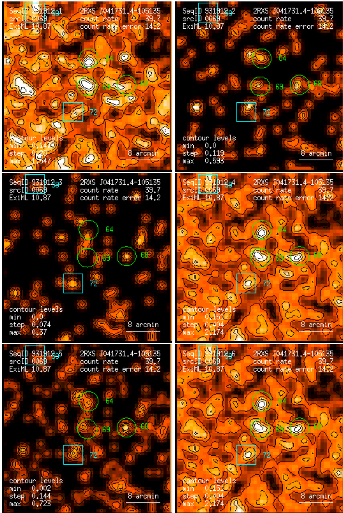
Figure 69: RASS 931912: detection 0069: band rate images, Gaussian filter: (1) PSPC channels 11 – 41, (2) 52 – 90, (3) 91 – 201, (4) 11 – 235, (5) 52 – 201, (6) 11 – 201. Broad band rates in counts/ks. Band rate contour levels in counts/ks/arcmin 2 .
