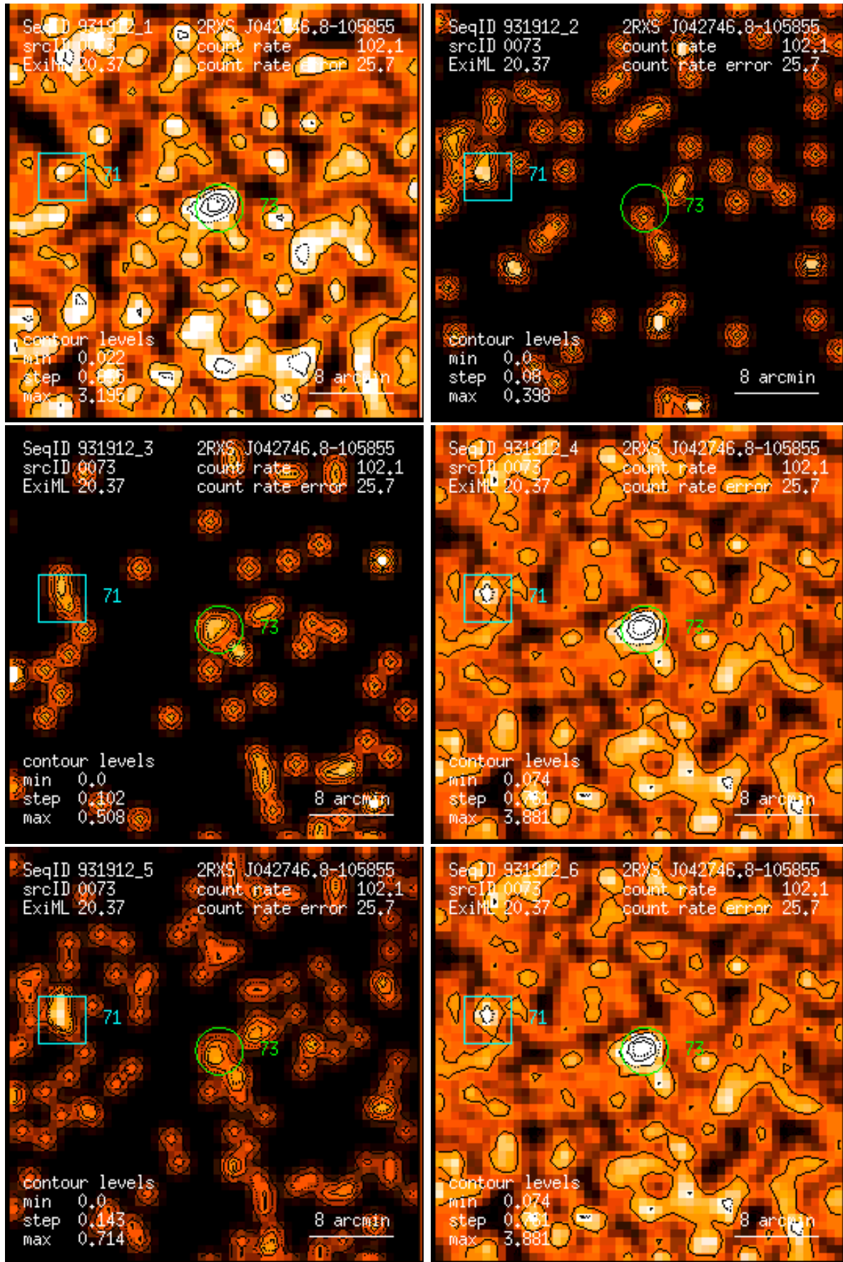
Figure 73: RASS 931912: detection 0073: band rate images, Gaussian filter: (1) PSPC channels 11 – 41, (2) 52 – 90, (3) 91 – 201, (4) 11 – 235, (5) 52 – 201, (6) 11 – 201. Broad band rates in counts/ks. Band rate contour levels in counts/ks/arcmin 2 .
