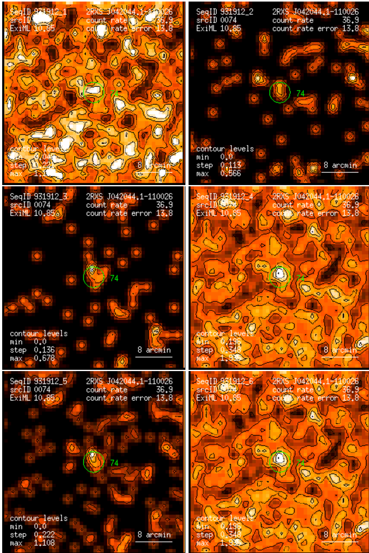
Figure 74: RASS 931912: detection 0074: band rate images, Gaussian filter: (1) PSPC channels 11 – 41, (2) 52 – 90, (3) 91 – 201, (4) 11 – 235, (5) 52 – 201, (6) 11 – 201. Broad band rates in counts/ks. Band rate contour levels in counts/ks/arcmin 2 .
