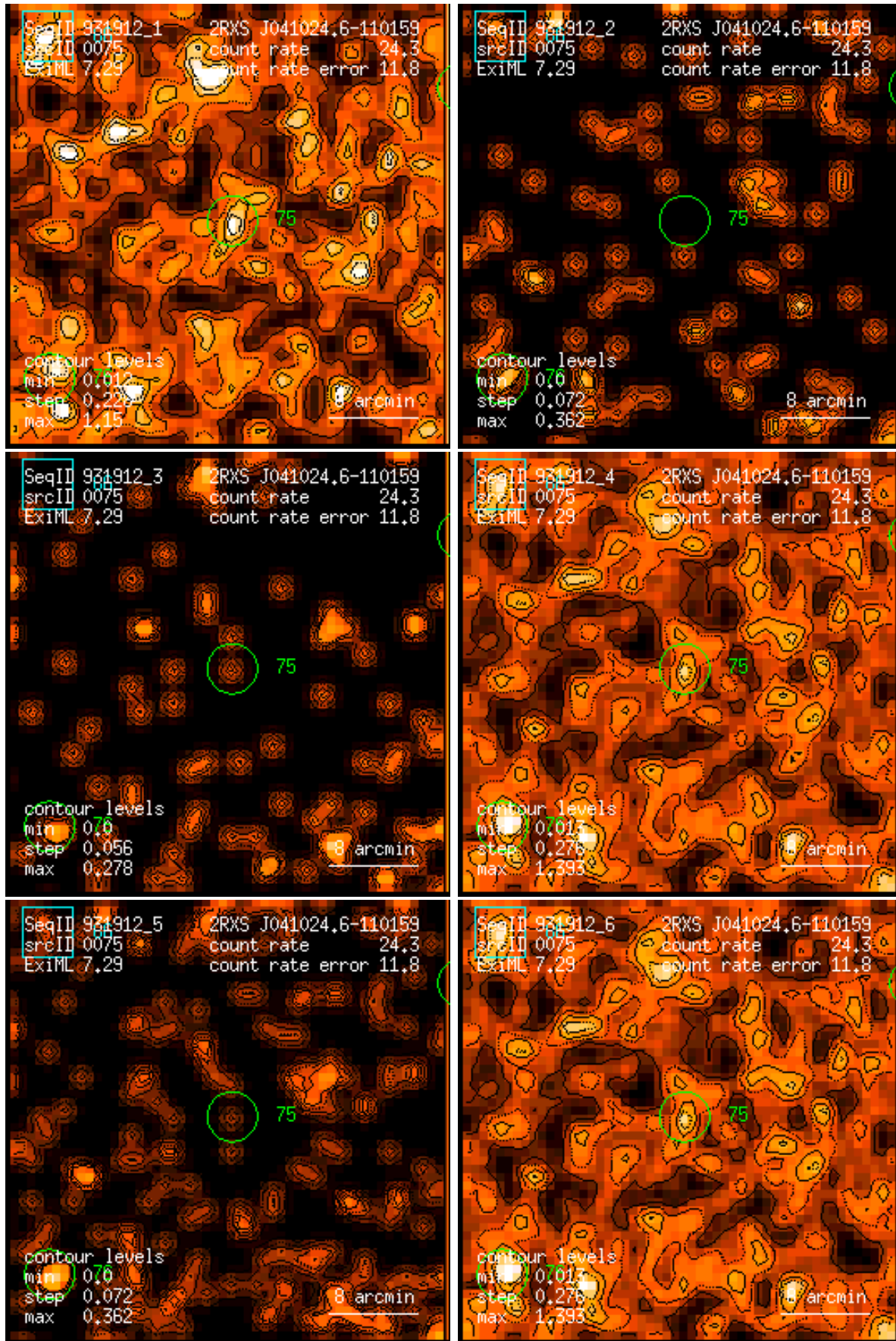
Figure 75: RASS 931912: detection 0075: band rate images, Gaussian filter: (1) PSPC channels 11 – 41, (2) 52 – 90, (3) 91 – 201, (4) 11 – 235, (5) 52 – 201, (6) 11 – 201. Broad band rates in counts/ks. Band rate contour levels in counts/ks/arcmin 2 .
