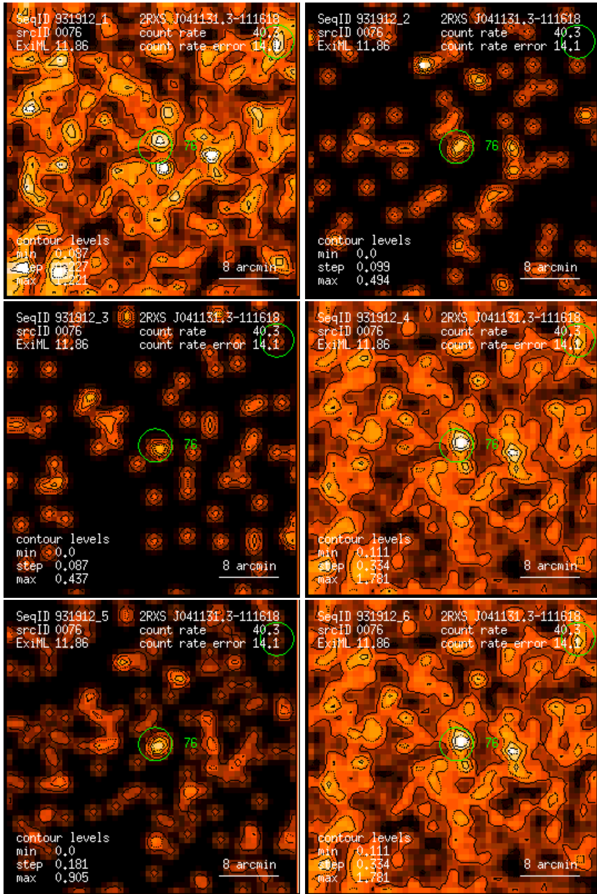
Figure 76: RASS 931912: detection 0076: band rate images, Gaussian filter: (1) PSPC channels 11 – 41, (2) 52 – 90, (3) 91 – 201, (4) 11 – 235, (5) 52 – 201, (6) 11 – 201. Broad band rates in counts/ks. Band rate contour levels in counts/ks/arcmin 2 .
