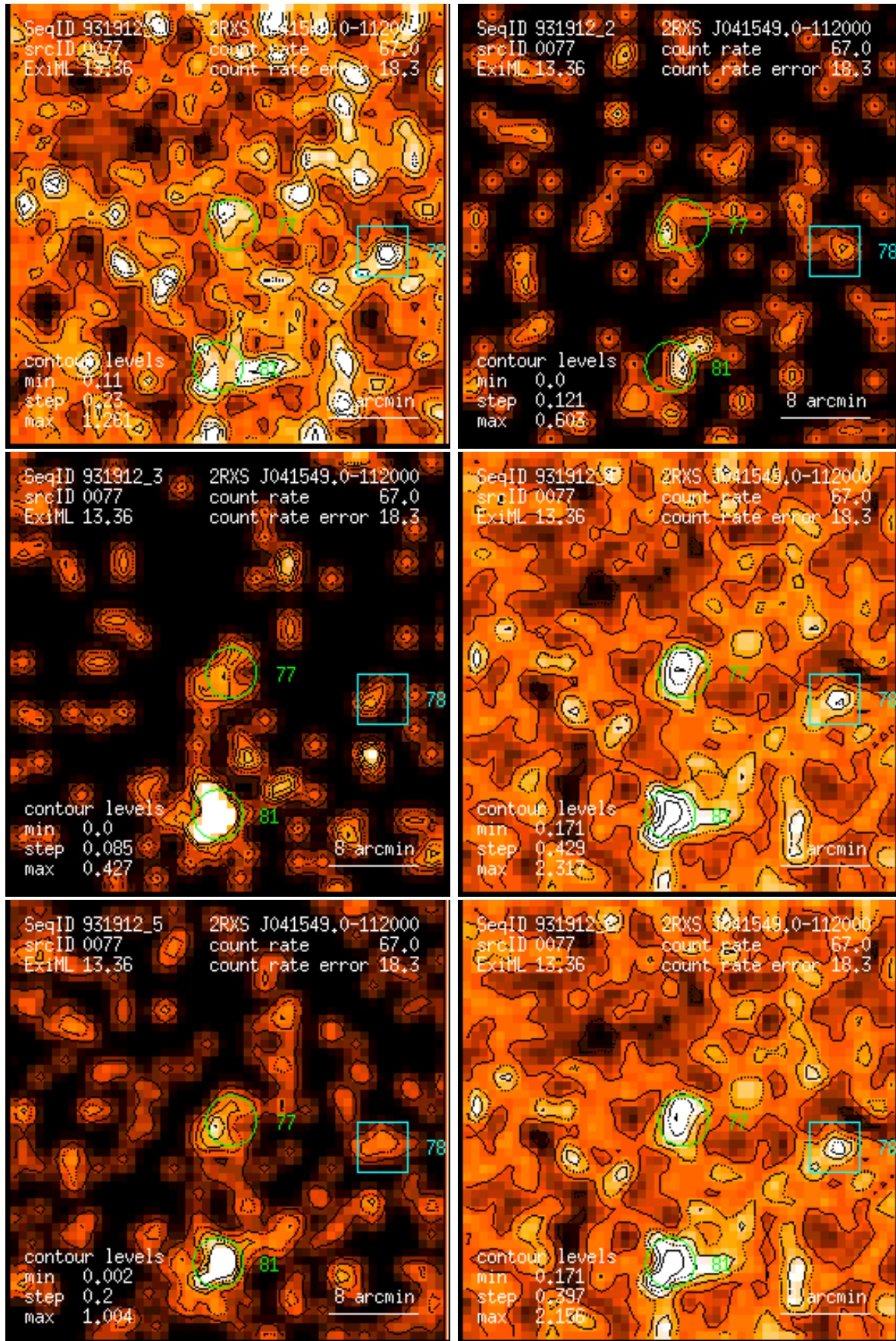
Figure 77: RASS 931912: detection 0077: band rate images, Gaussian filter: (1) PSPC channels 11 – 41, (2) 52 – 90, (3) 91 – 201, (4) 11 – 235, (5) 52 – 201, (6) 11 – 201. Broad band rates in counts/ks. Band rate contour levels in counts/ks/arcmin 2 .
