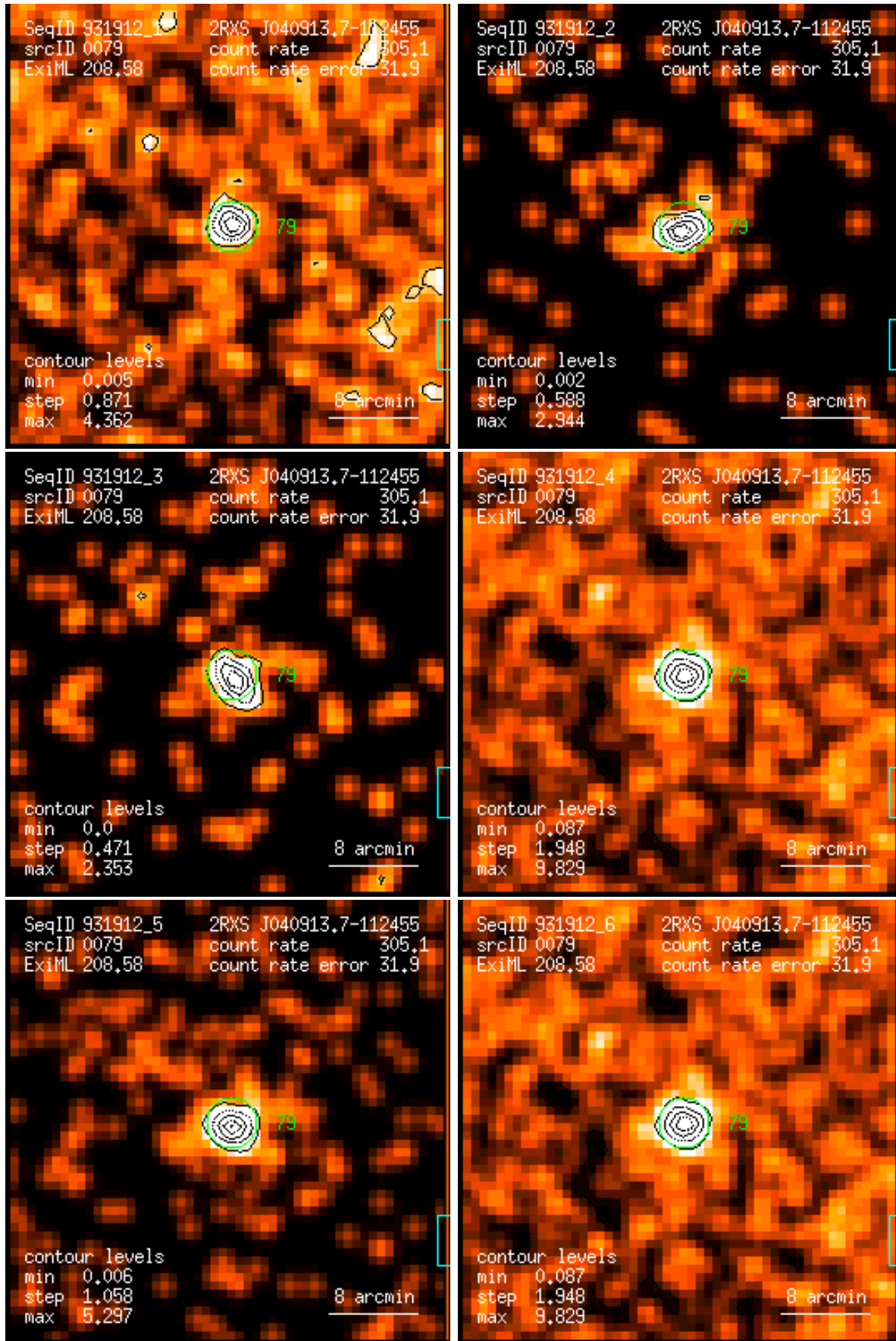
Figure 79: RASS 931912: detection 0079: band rate images, Gaussian filter: (1) PSPC channels 11 – 41, (2) 52 – 90, (3) 91 – 201, (4) 11 – 235, (5) 52 – 201, (6) 11 – 201. Broad band rates in counts/ks. Band rate contour levels in counts/ks/arcmin 2 .
