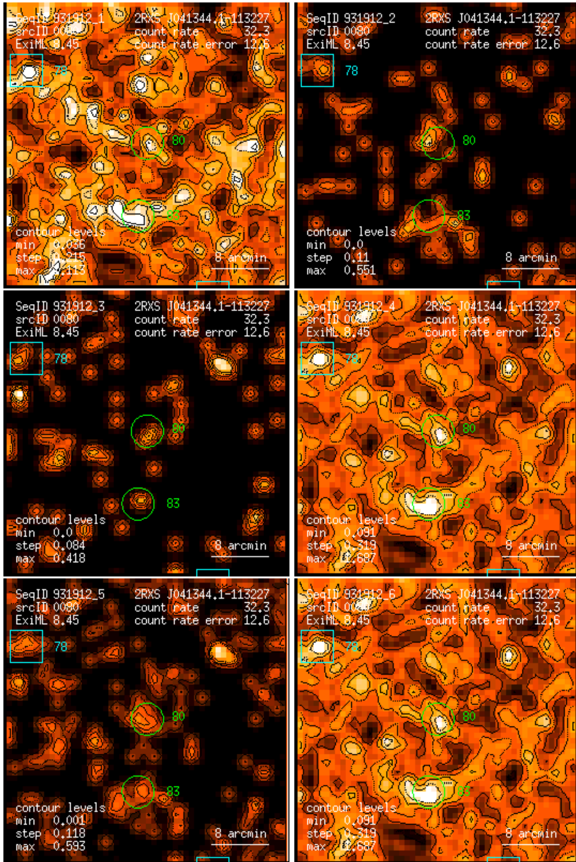
Figure 80: RASS 931912: detection 0080: band rate images, Gaussian filter: (1) PSPC channels 11 – 41, (2) 52 – 90, (3) 91 – 201, (4) 11 – 235, (5) 52 – 201, (6) 11 – 201. Broad band rates in counts/ks. Band rate contour levels in counts/ks/arcmin 2 .
