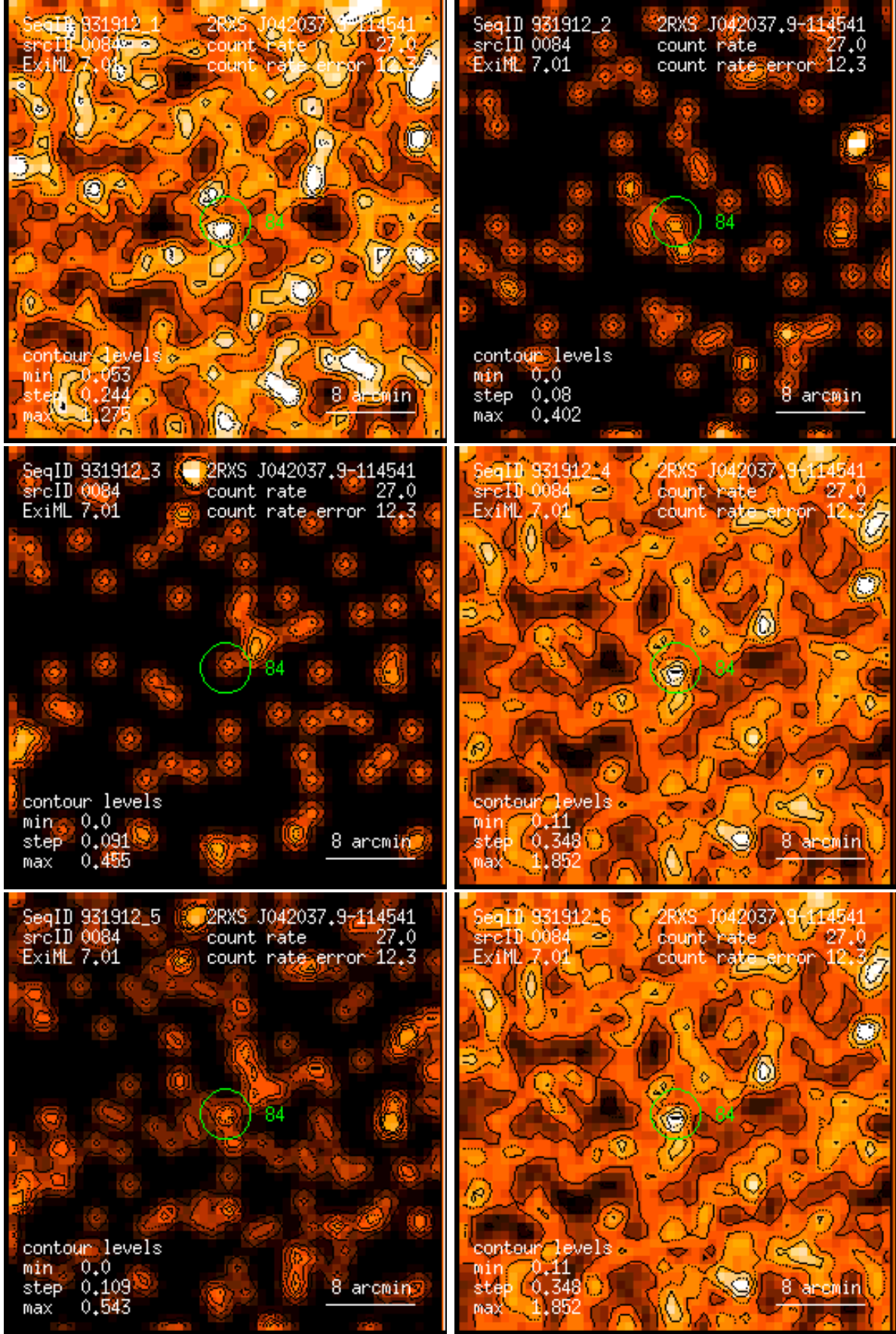
Figure 84: RASS 931912: detection 0084: band rate images, Gaussian filter: (1) PSPC channels 11 – 41, (2) 52 – 90, (3) 91 – 201, (4) 11 – 235, (5) 52 – 201, (6) 11 – 201. Broad band rates in counts/ks. Band rate contour levels in counts/ks/arcmin 2 .
