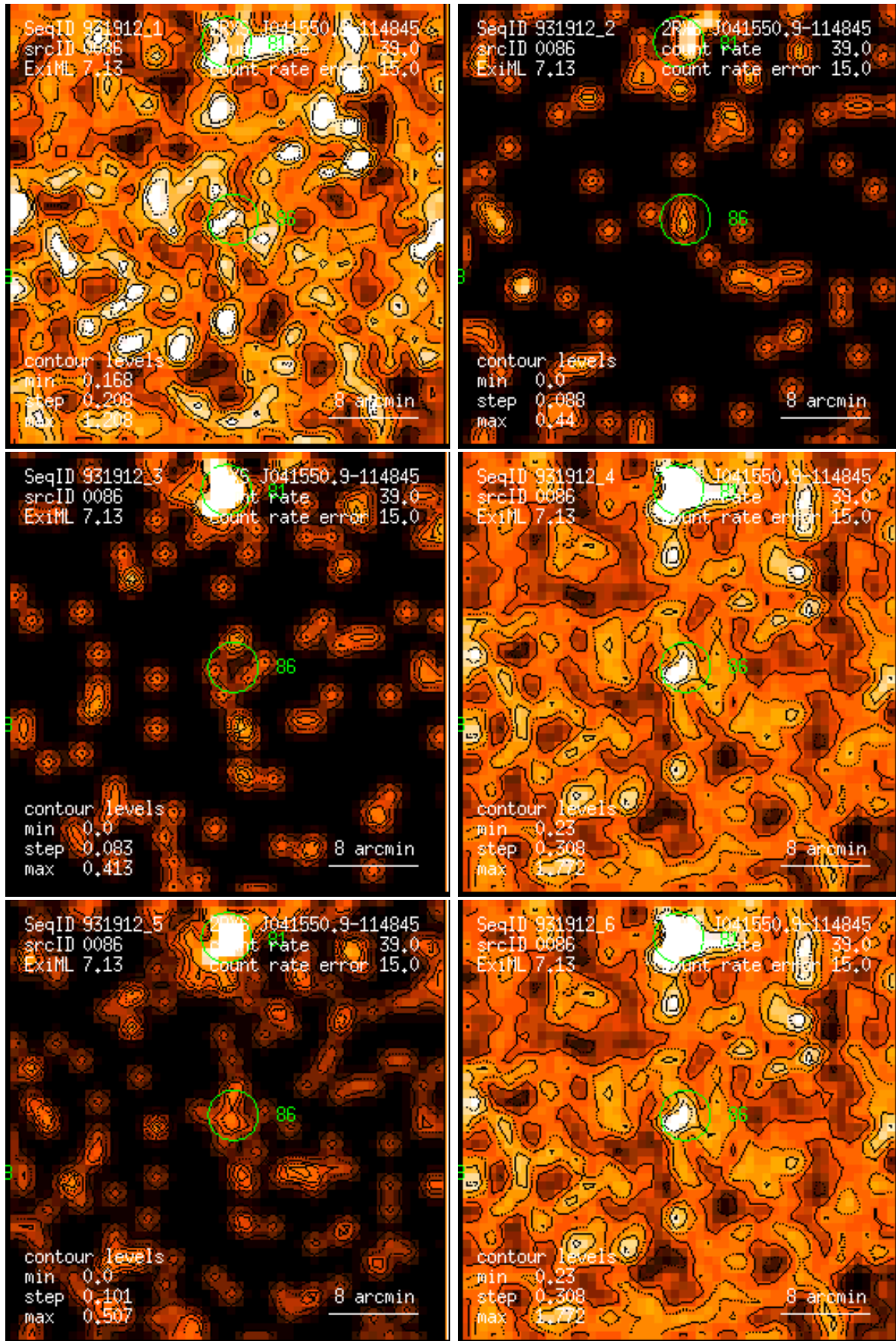
Figure 86: RASS 931912: detection 0086: band rate images, Gaussian filter: (1) PSPC channels 11 – 41, (2) 52 – 90, (3) 91 – 201, (4) 11 – 235, (5) 52 – 201, (6) 11 – 201. Broad band rates in counts/ks. Band rate contour levels in counts/ks/arcmin 2 .
