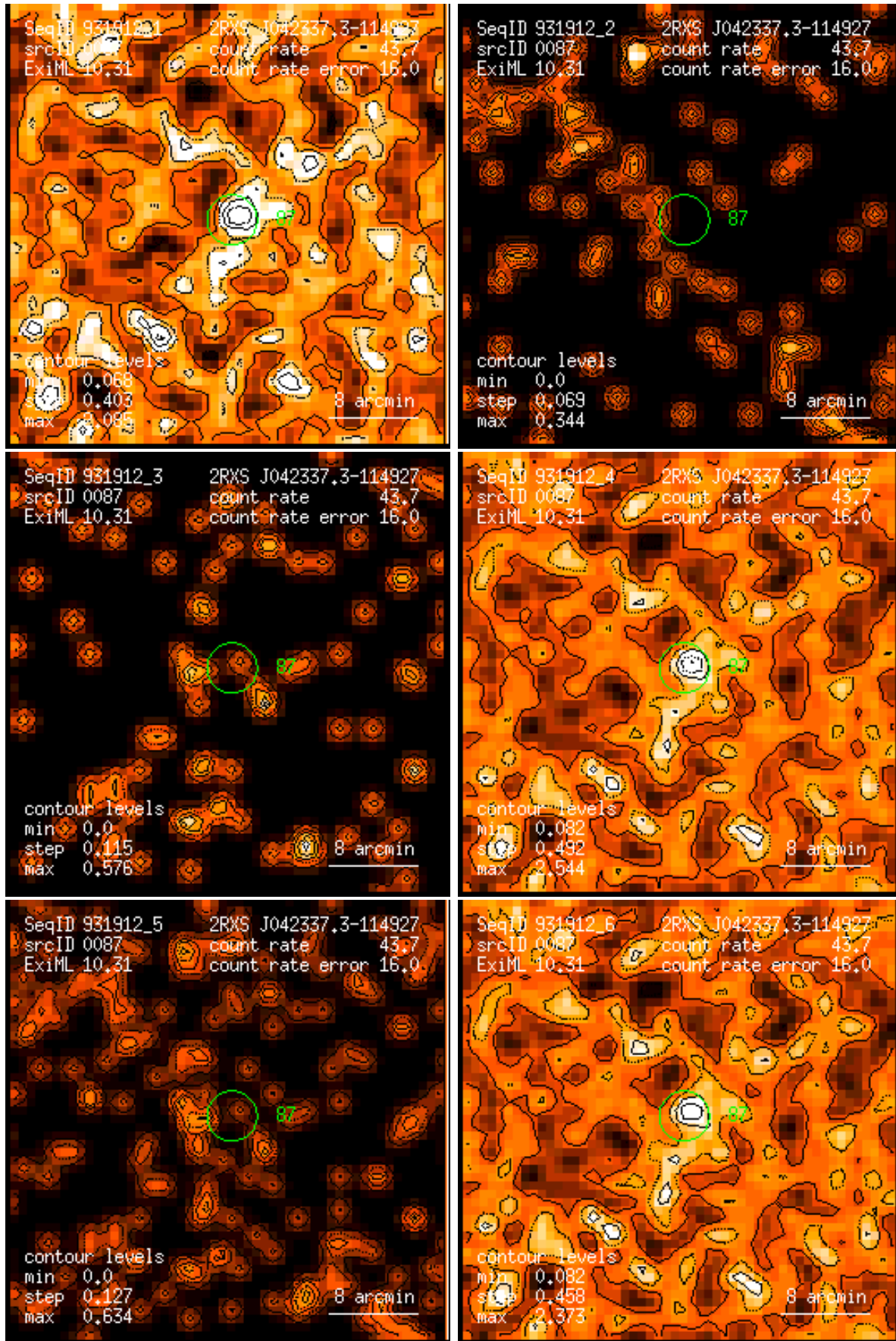
Figure 87: RASS 931912: detection 0087: band rate images, Gaussian filter: (1) PSPC channels 11 – 41, (2) 52 – 90, (3) 91 – 201, (4) 11 – 235, (5) 52 – 201, (6) 11 – 201. Broad band rates in counts/ks. Band rate contour levels in counts/ks/arcmin 2 .
