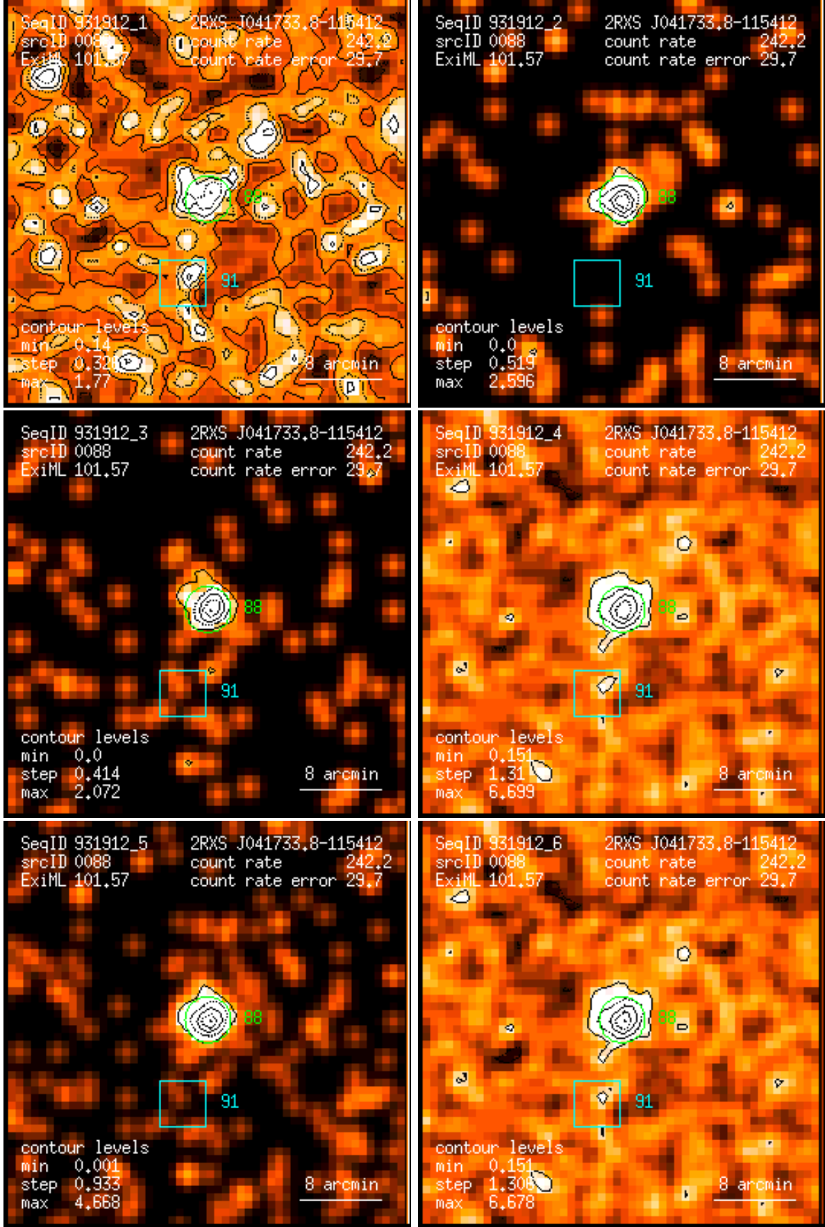
Figure 88: RASS 931912: detection 0088: band rate images, Gaussian filter: (1) PSPC channels 11 – 41, (2) 52 – 90, (3) 91 – 201, (4) 11 – 235, (5) 52 – 201, (6) 11 – 201. Broad band rates in counts/ks. Band rate contour levels in counts/ks/arcmin 2 .
