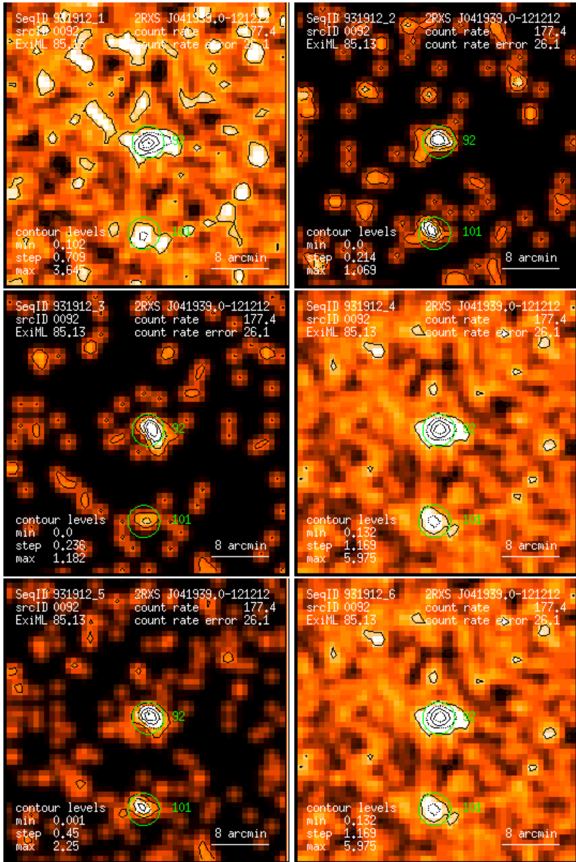
Figure 92: RASS 931912: detection 0092: band rate images, Gaussian filter: (1) PSPC channels 11 – 41, (2) 52 – 90, (3) 91 – 201, (4) 11 – 235, (5) 52 – 201, (6) 11 – 201. Broad band rates in counts/ks. Band rate contour levels in counts/ks/arcmin 2 .
