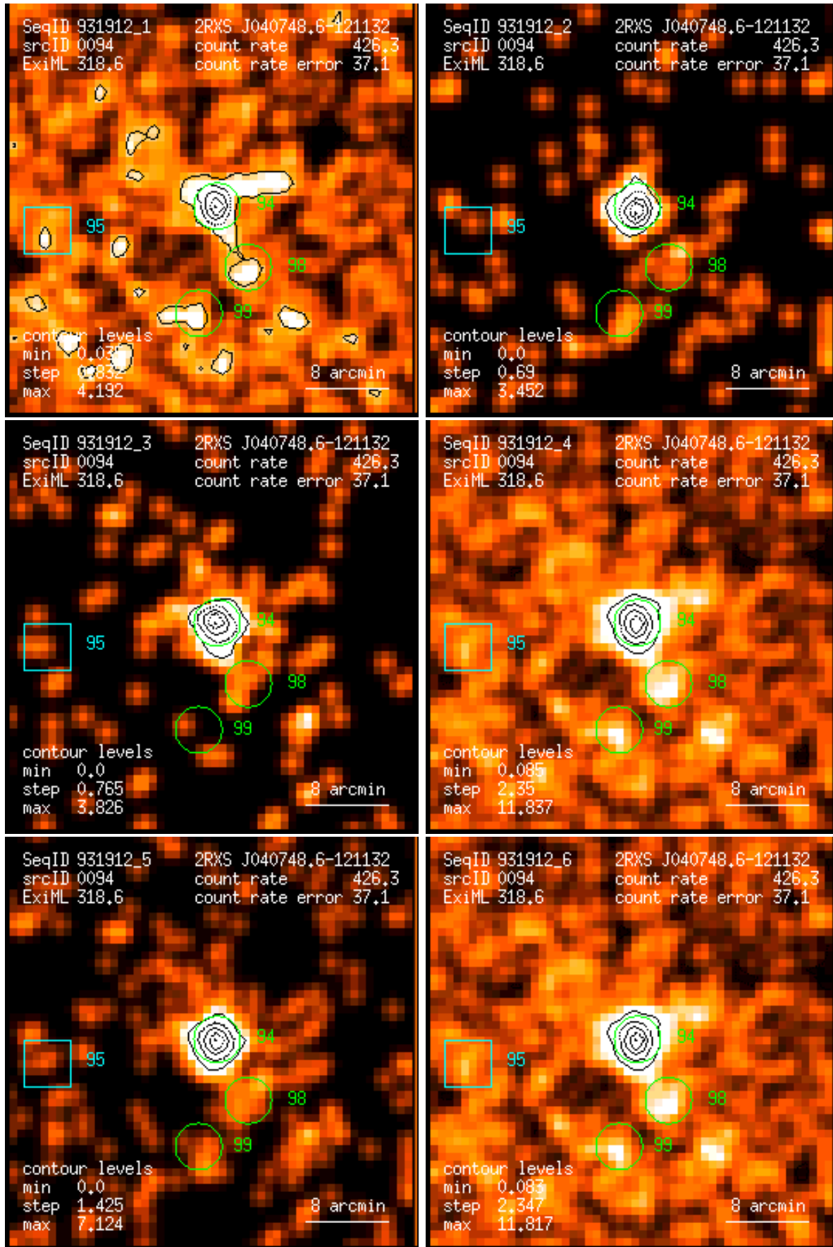
Figure 94: RASS 931912: detection 0094: band rate images, Gaussian filter: (1) PSPC channels 11 – 41, (2) 52 – 90, (3) 91 – 201, (4) 11 – 235, (5) 52 – 201, (6) 11 – 201. Broad band rates in counts/ks. Band rate contour levels in counts/ks/arcmin 2 .
