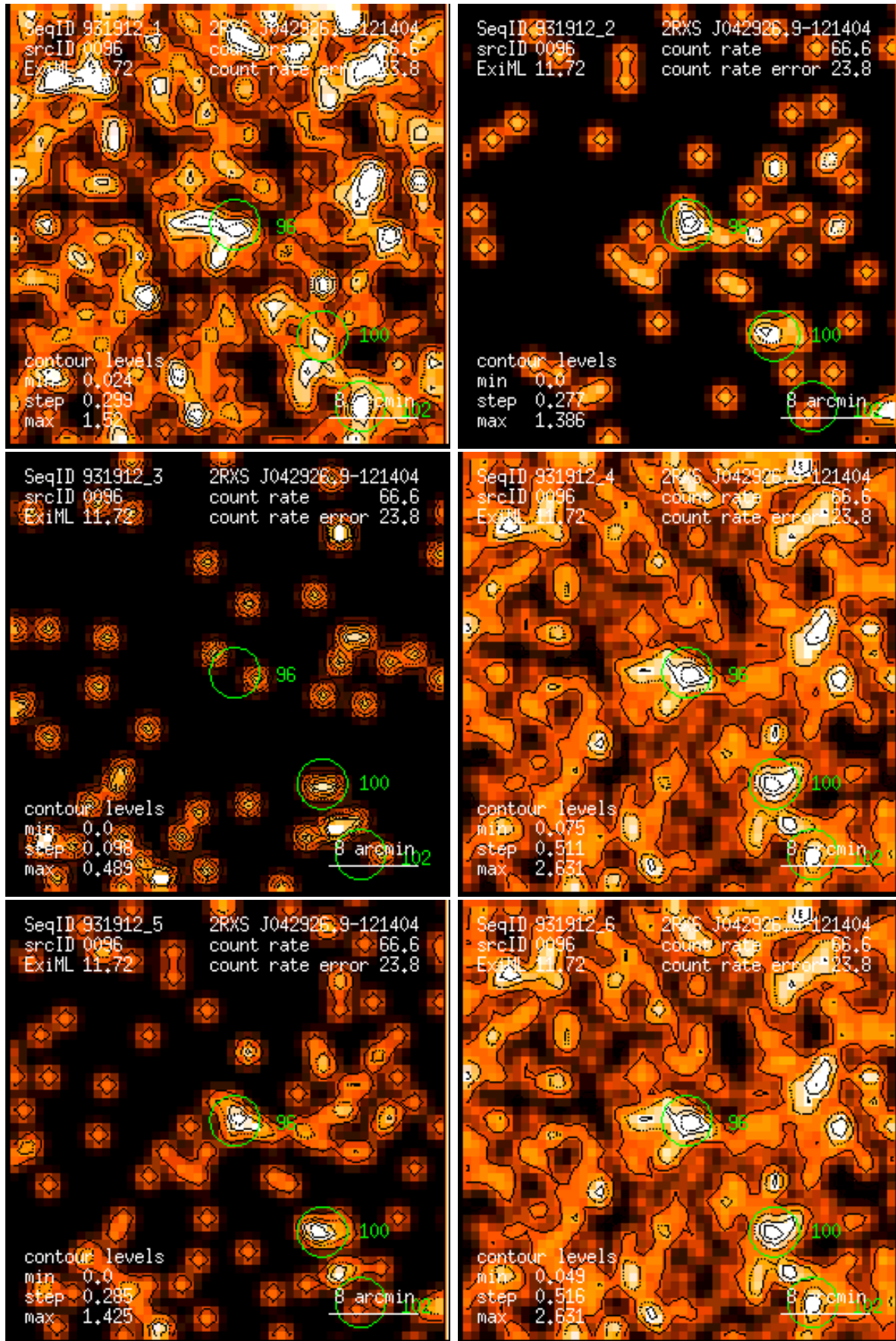
Figure 96: RASS 931912: detection 0096: band rate images, Gaussian filter: (1) PSPC channels 11 – 41, (2) 52 – 90, (3) 91 – 201, (4) 11 – 235, (5) 52 – 201, (6) 11 – 201. Broad band rates in counts/ks. Band rate contour levels in counts/ks/arcmin 2 .
