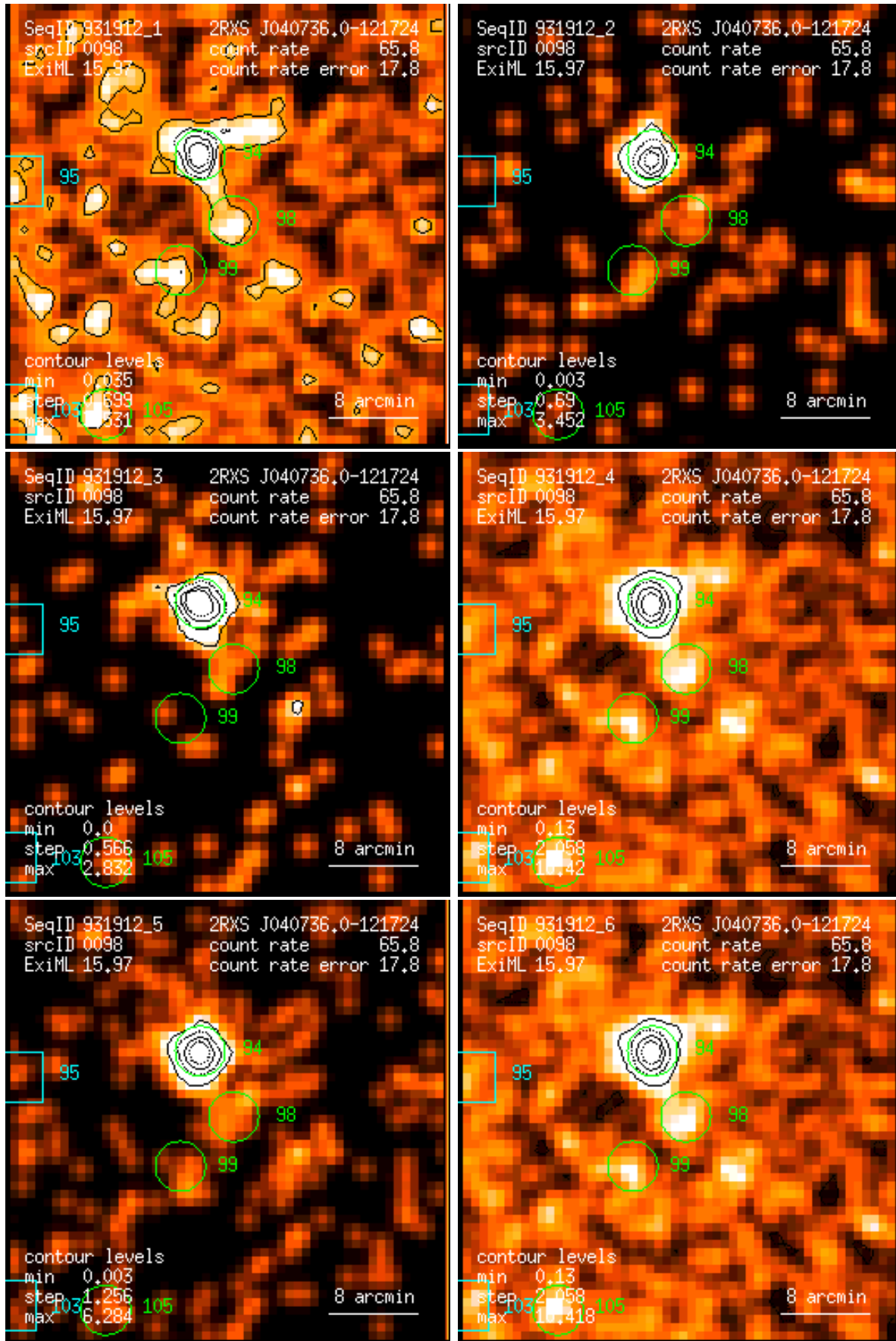
Figure 98: RASS 931912: detection 0098: band rate images, Gaussian filter: (1) PSPC channels 11 – 41, (2) 52 – 90, (3) 91 – 201, (4) 11 – 235, (5) 52 – 201, (6) 11 – 201. Broad band rates in counts/ks. Band rate contour levels in counts/ks/arcmin 2 .
