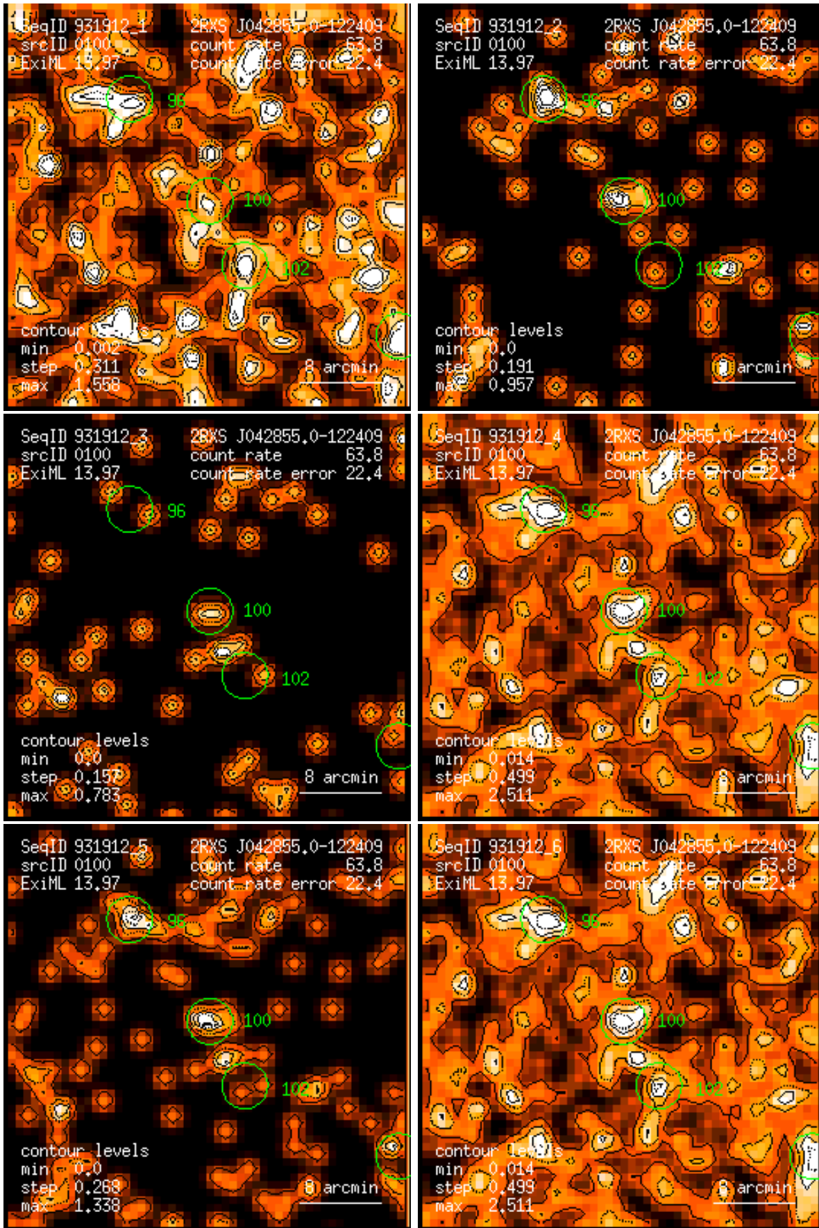
Figure 100: RASS 931912: detection 0100: band rate images, Gaussian filter: (1) PSPC channels 11 – 41, (2) 52 – 90, (3) 91 – 201, (4) 11 – 235, (5) 52 – 201, (6) 11 – 201. Broad band rates in counts/ks. Band rate contour levels in counts/ks/arcmin 2 .
