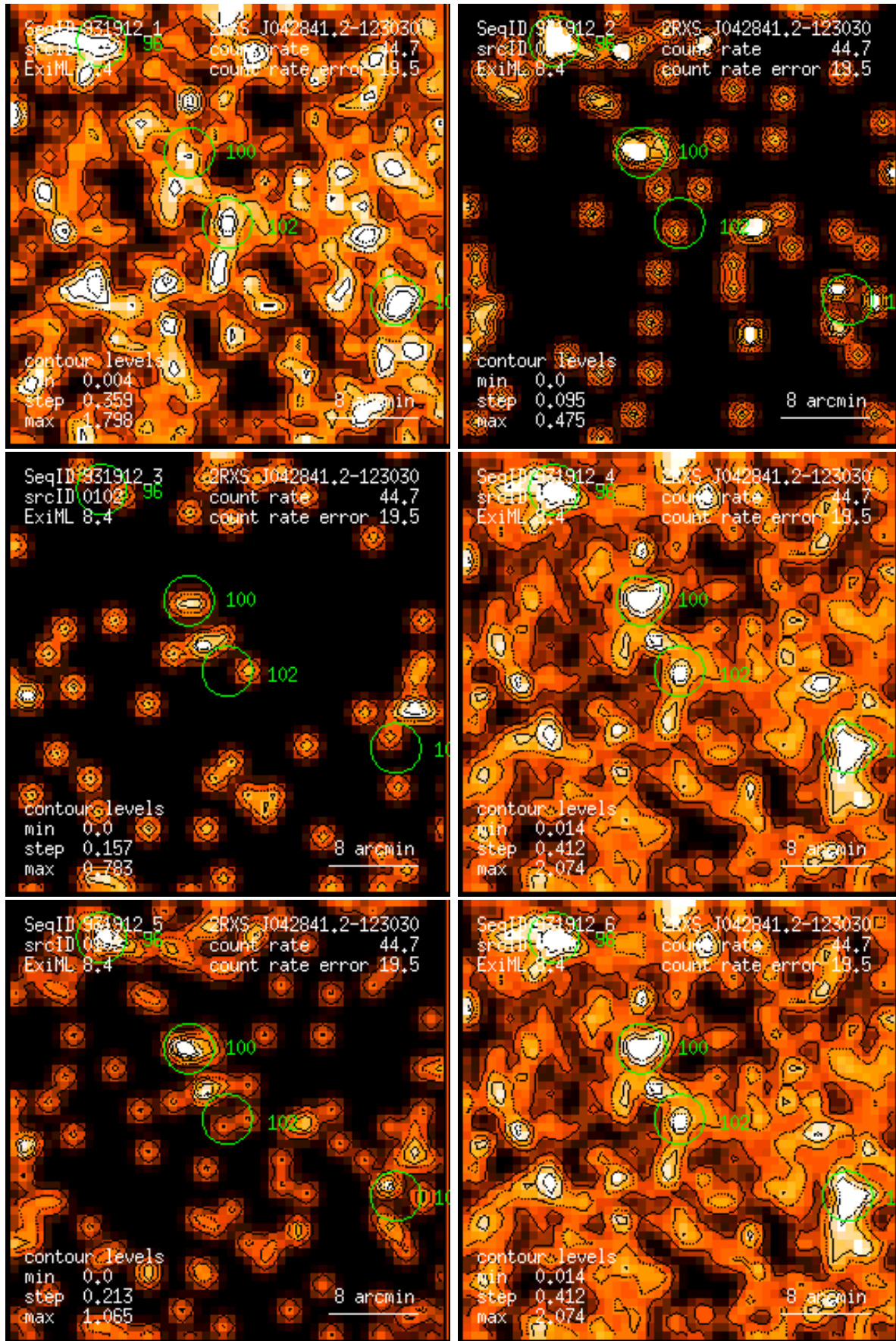
Figure 102: RASS 931912: detection 0102: band rate images, Gaussian filter: (1) PSPC channels 11 – 41, (2) 52 – 90, (3) 91 – 201, (4) 11 – 235, (5) 52 – 201, (6) 11 – 201. Broad band rates in counts/ks. Band rate contour levels in counts/ks/arcmin 2 .
