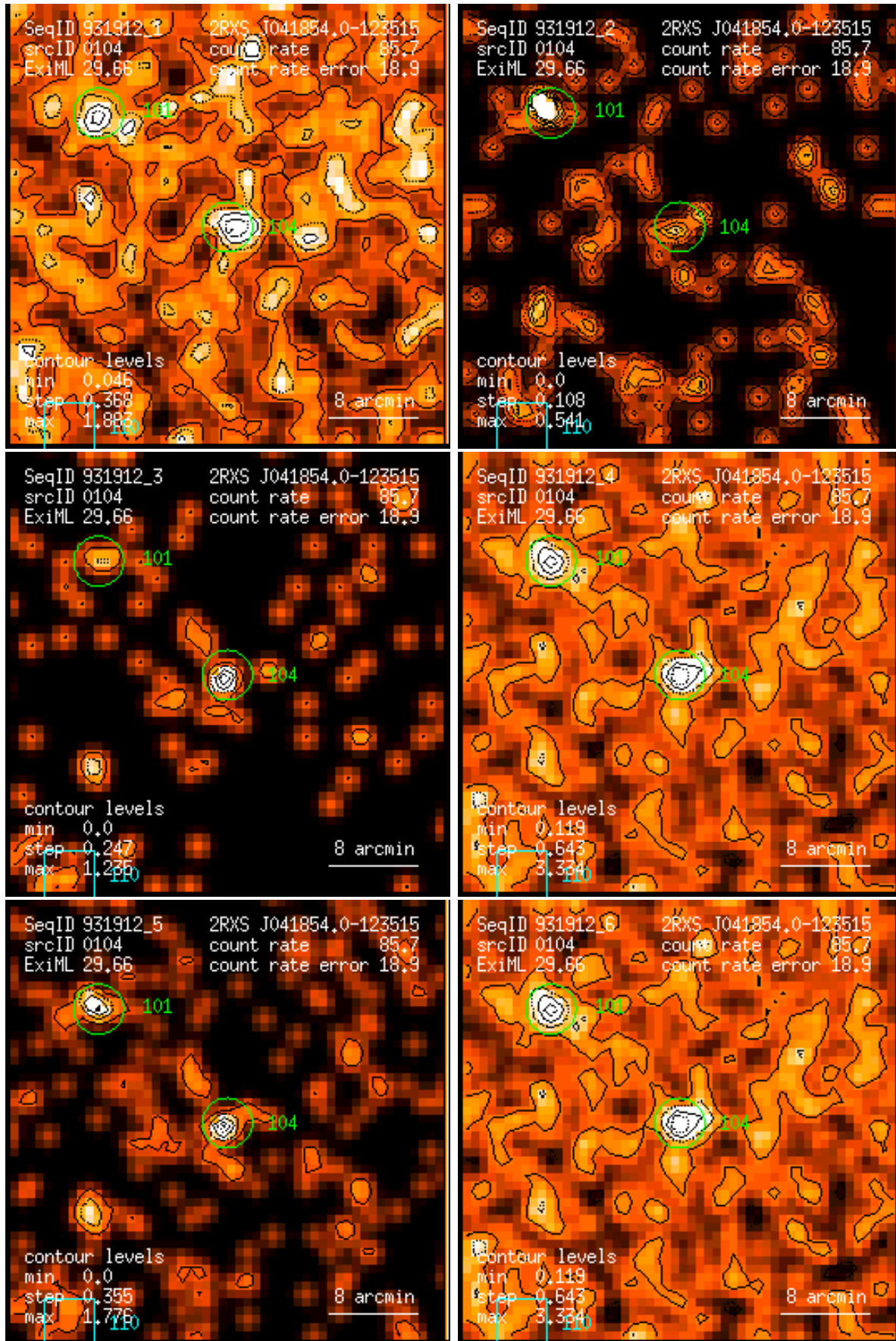
Figure 104: RASS 931912: detection 0104: band rate images, Gaussian filter: (1) PSPC channels 11 – 41, (2) 52 – 90, (3) 91 – 201, (4) 11 – 235, (5) 52 – 201, (6) 11 – 201. Broad band rates in counts/ks. Band rate contour levels in counts/ks/arcmin 2 .
