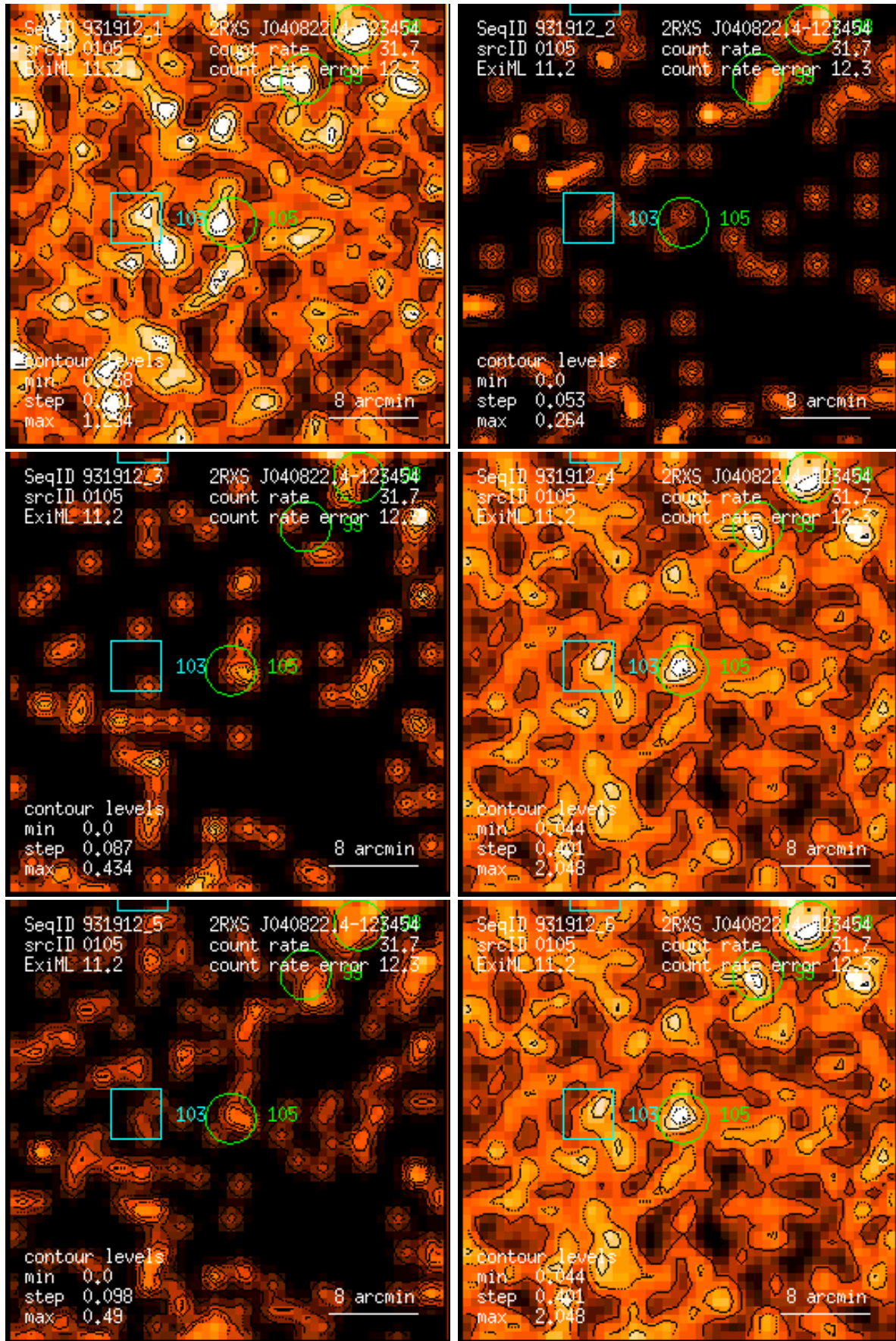
Figure 105: RASS 931912: detection 0105: band rate images, Gaussian filter: (1) PSPC channels 11 – 41, (2) 52 – 90, (3) 91 – 201, (4) 11 – 235, (5) 52 – 201, (6) 11 – 201. Broad band rates in counts/ks. Band rate contour levels in counts/ks/arcmin 2 .
