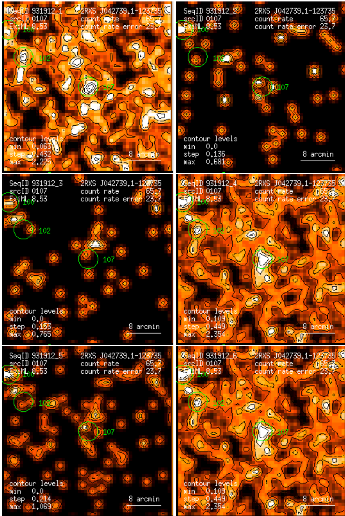
Figure 107: RASS 931912: detection 0107: band rate images, Gaussian filter: (1) PSPC channels 11 – 41, (2) 52 – 90, (3) 91 – 201, (4) 11 – 235, (5) 52 – 201, (6) 11 – 201. Broad band rates in counts/ks. Band rate contour levels in counts/ks/arcmin 2 .
