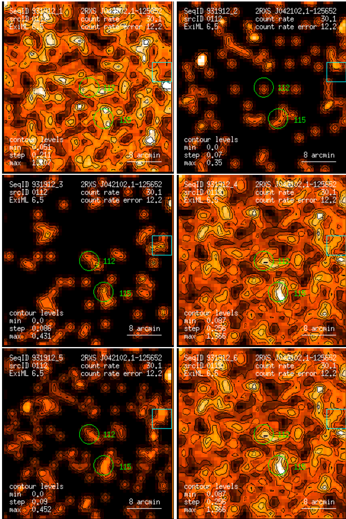
Figure 112: RASS 931912: detection 0112: band rate images, Gaussian filter: (1) PSPC channels 11 – 41, (2) 52 – 90, (3) 91 – 201, (4) 11 – 235, (5) 52 – 201, (6) 11 – 201. Broad band rates in counts/ks. Band rate contour levels in counts/ks/arcmin 2 .
