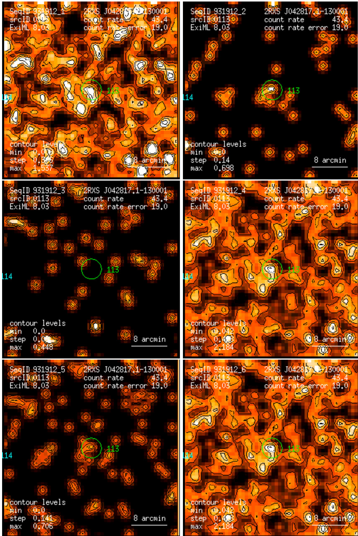
Figure 113: RASS 931912: detection 0113: band rate images, Gaussian filter: (1) PSPC channels 11 – 41, (2) 52 – 90, (3) 91 – 201, (4) 11 – 235, (5) 52 – 201, (6) 11 – 201. Broad band rates in counts/ks. Band rate contour levels in counts/ks/arcmin 2 .
