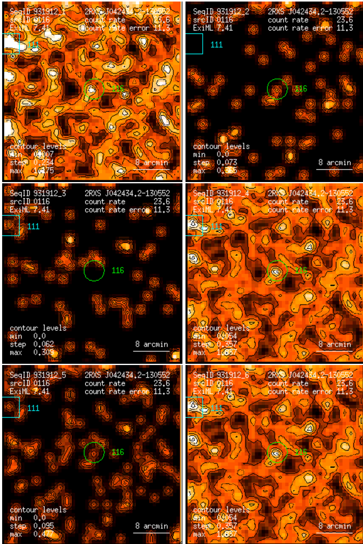
Figure 116: RASS 931912: detection 0116: band rate images, Gaussian filter: (1) PSPC channels 11 – 41, (2) 52 – 90, (3) 91 – 201, (4) 11 – 235, (5) 52 – 201, (6) 11 – 201. Broad band rates in counts/ks. Band rate contour levels in counts/ks/arcmin 2 .
