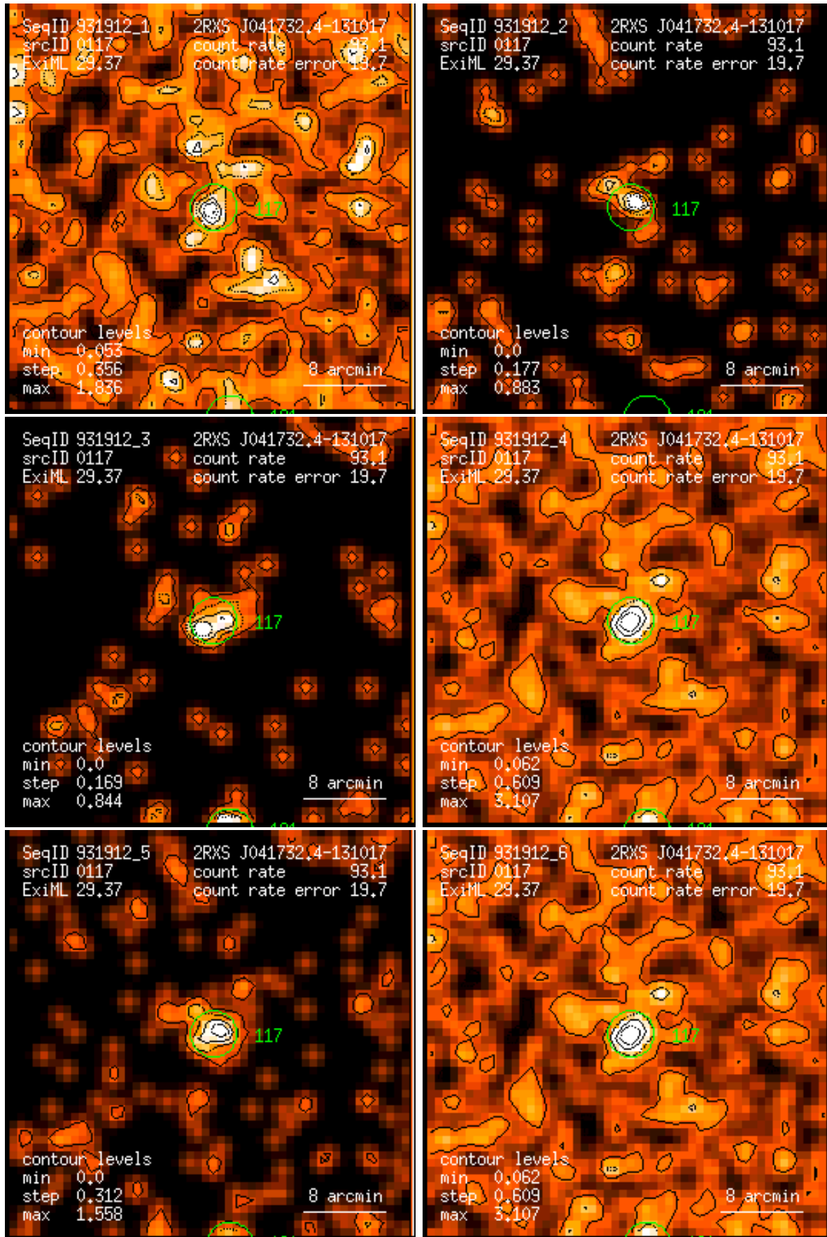
Figure 117: RASS 931912: detection 0117: band rate images, Gaussian filter: (1) PSPC channels 11 – 41, (2) 52 – 90, (3) 91 – 201, (4) 11 – 235, (5) 52 – 201, (6) 11 – 201. Broad band rates in counts/ks. Band rate contour levels in counts/ks/arcmin 2 .
