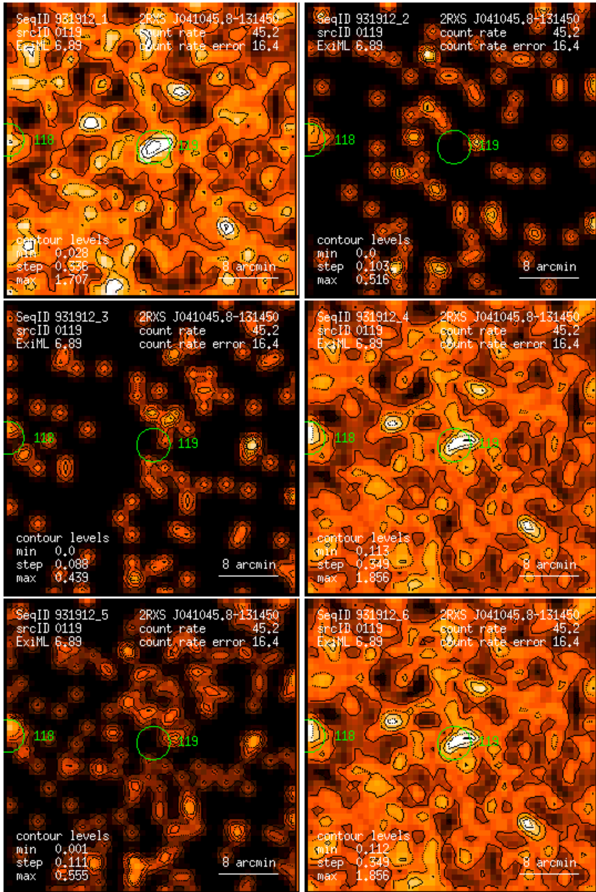
Figure 119: RASS 931912: detection 0119: band rate images, Gaussian filter: (1) PSPC channels 11 – 41, (2) 52 – 90, (3) 91 – 201, (4) 11 – 235, (5) 52 – 201, (6) 11 – 201. Broad band rates in counts/ks. Band rate contour levels in counts/ks/arcmin 2 .
