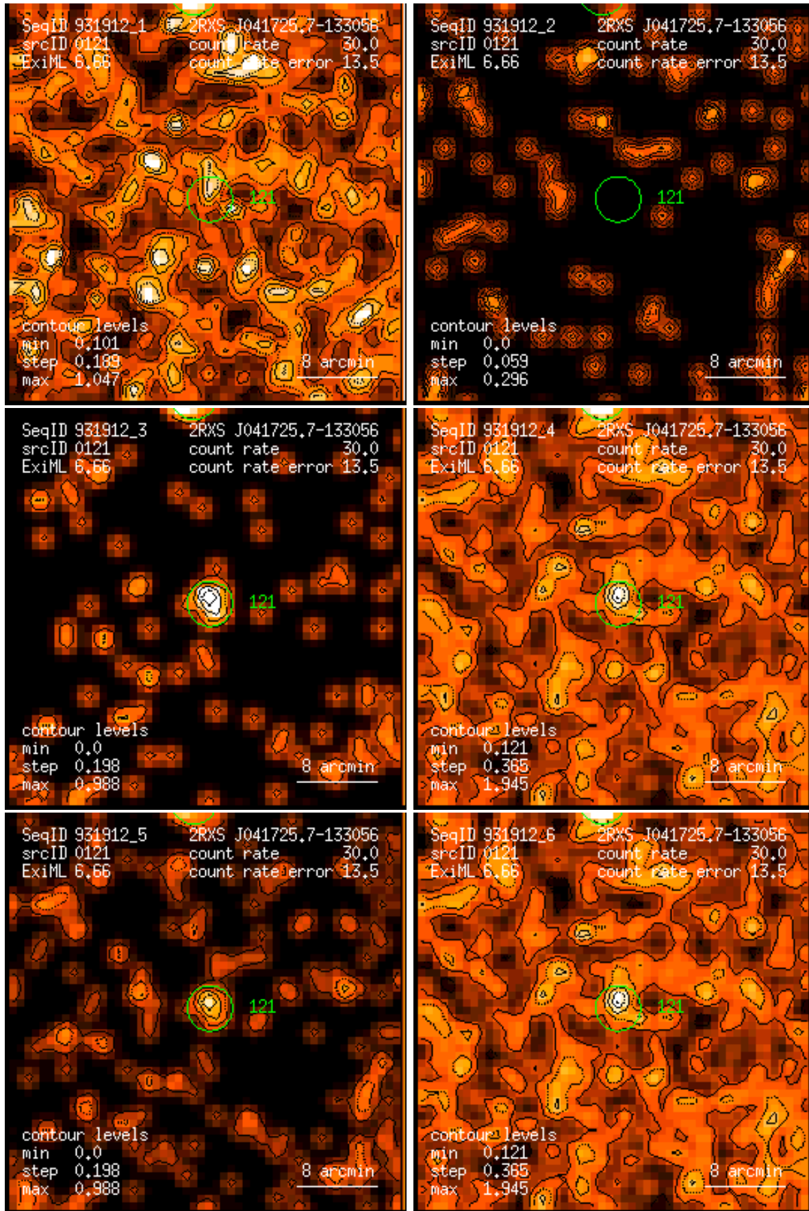
Figure 121: RASS 931912: detection 0121: band rate images, Gaussian filter: (1) PSPC channels 11 – 41, (2) 52 – 90, (3) 91 – 201, (4) 11 – 235, (5) 52 – 201, (6) 11 – 201. Broad band rates in counts/ks. Band rate contour levels in counts/ks/arcmin 2 .
