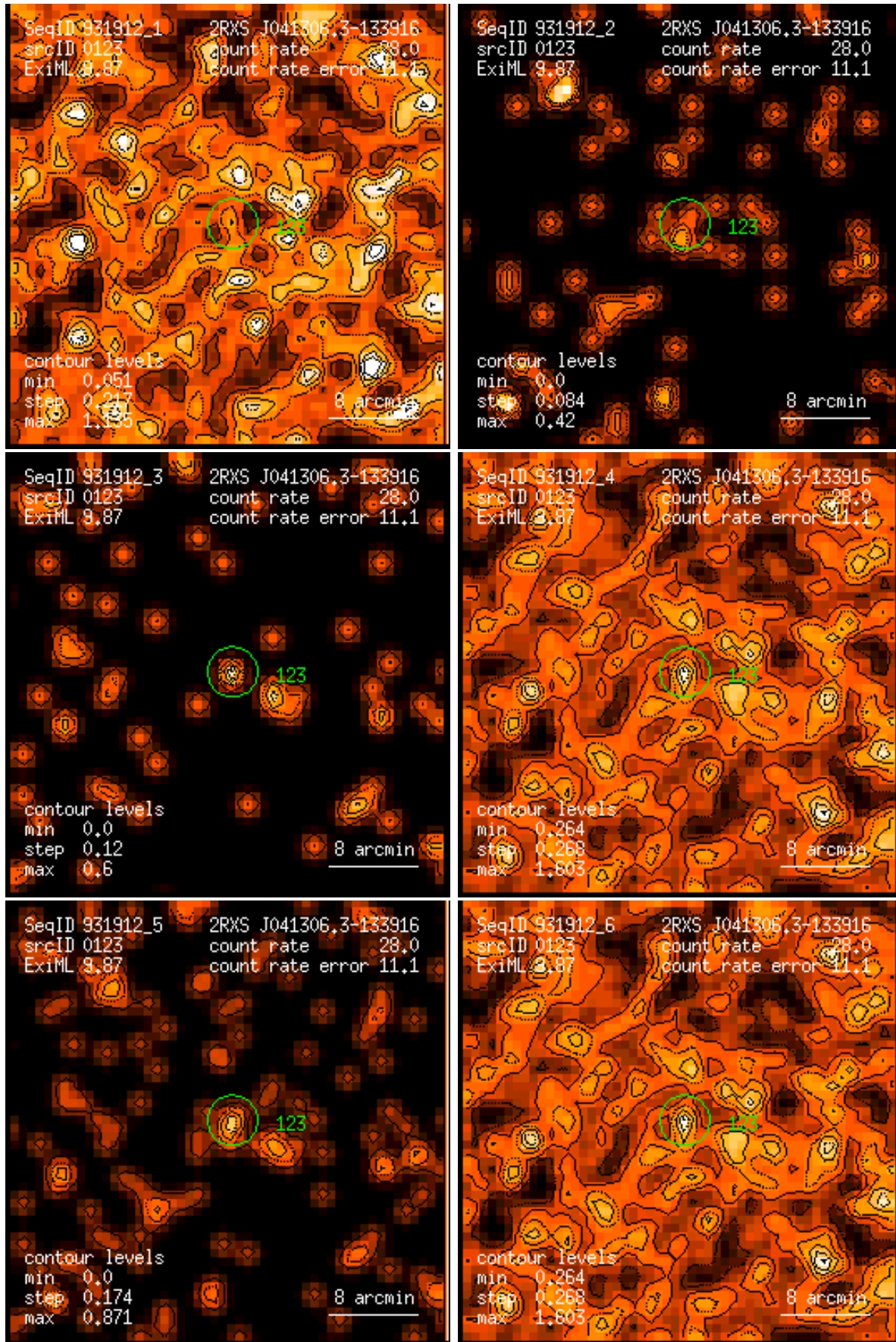
Figure 123: RASS 931912: detection 0123: band rate images, Gaussian filter: (1) PSPC channels 11 – 41, (2) 52 – 90, (3) 91 – 201, (4) 11 – 235, (5) 52 – 201, (6) 11 – 201. Broad band rates in counts/ks. Band rate contour levels in counts/ks/arcmin 2 .
