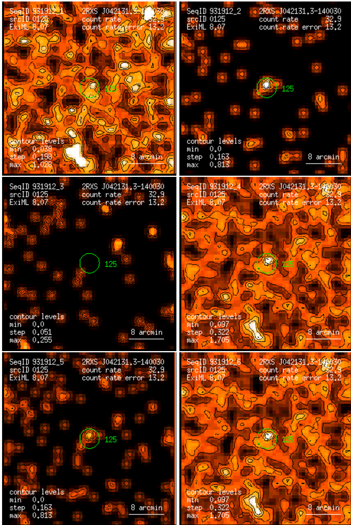
Figure 125: RASS 931912: detection 0125: band rate images, Gaussian filter: (1) PSPC channels 11 – 41, (2) 52 – 90, (3) 91 – 201, (4) 11 – 235, (5) 52 – 201, (6) 11 – 201. Broad band rates in counts/ks. Band rate contour levels in counts/ks/arcmin 2 .
