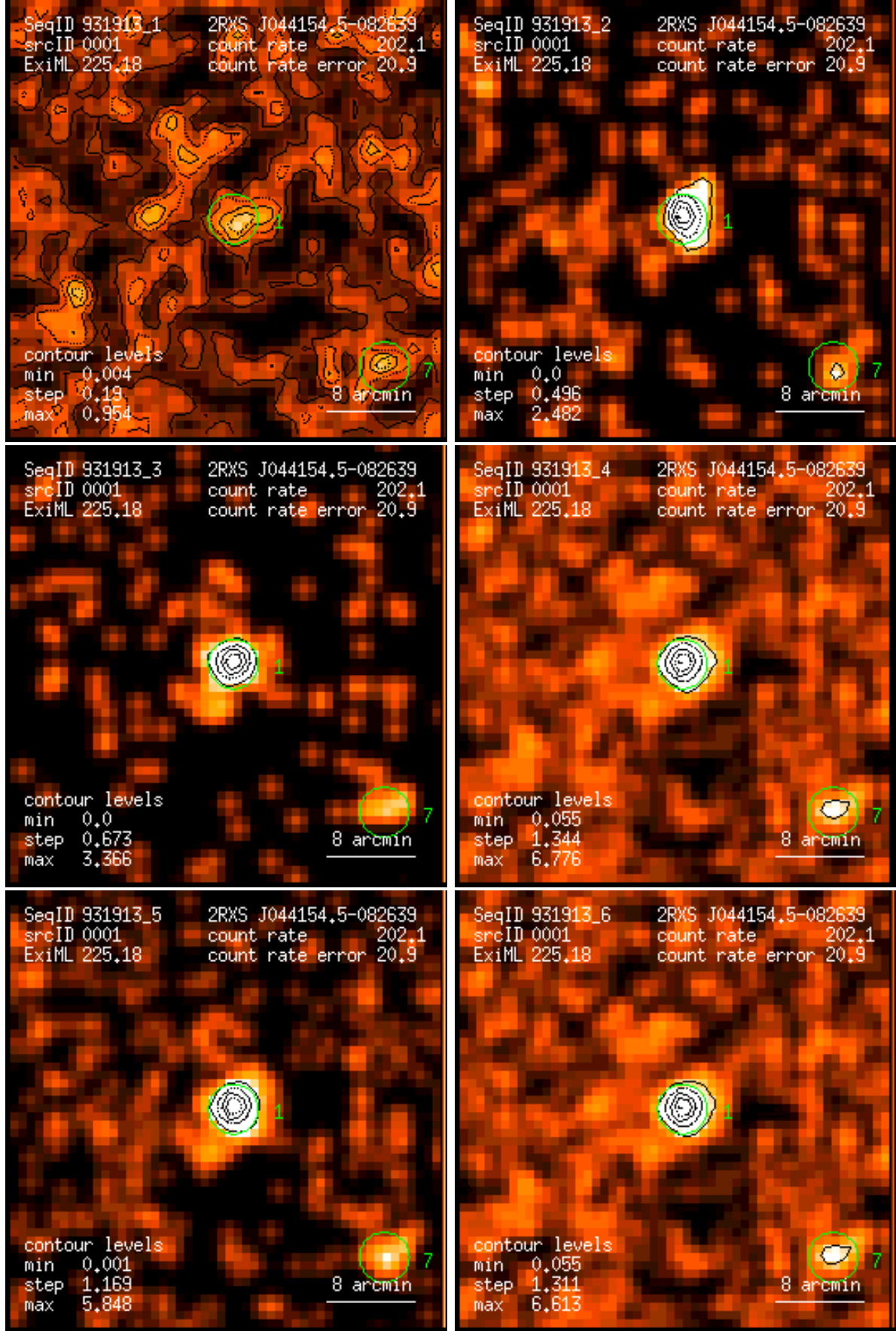
Figure 1: RASS 931913: detection 0001: band rate images, Gaussian filter: (1) PSPC channels 11 – 41, (2) 52 – 90, (3) 91 – 201, (4) 11 – 235, (5) 52 – 201, (6) 11 – 201. Broad band rates in counts/ks. Band rate contour levels in counts/ks/arcmin 2 .
