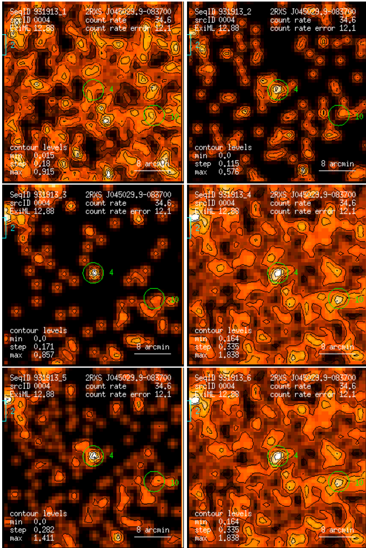
Figure 4: RASS 931913: detection 0004: band rate images, Gaussian filter: (1) PSPC channels 11 – 41, (2) 52 – 90, (3) 91 – 201, (4) 11 – 235, (5) 52 – 201, (6) 11 – 201. Broad band rates in counts/ks. Band rate contour levels in counts/ks/arcmin 2 .
