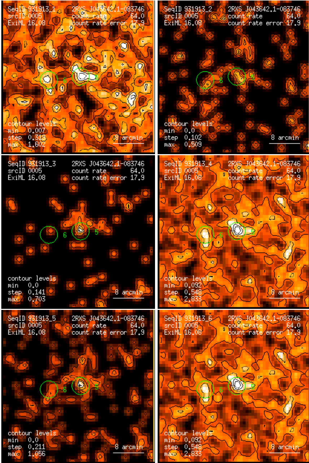
Figure 5: RASS 931913: detection 0005: band rate images, Gaussian filter: (1) PSPC channels 11 – 41, (2) 52 – 90, (3) 91 – 201, (4) 11 – 235, (5) 52 – 201, (6) 11 – 201. Broad band rates in counts/ks. Band rate contour levels in counts/ks/arcmin 2 .
