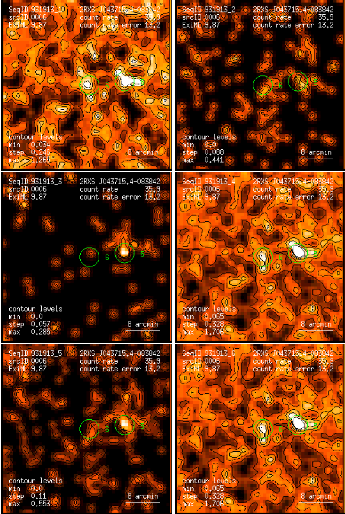
Figure 6: RASS 931913: detection 0006: band rate images, Gaussian filter: (1) PSPC channels 11 – 41, (2) 52 – 90, (3) 91 – 201, (4) 11 – 235, (5) 52 – 201, (6) 11 – 201. Broad band rates in counts/ks. Band rate contour levels in counts/ks/arcmin 2 .
