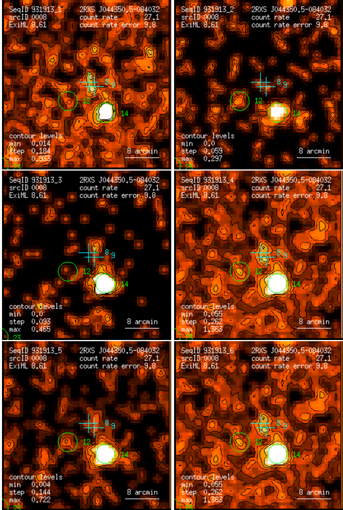
Figure 8: RASS 931913: detection 0008: band rate images, Gaussian filter: (1) PSPC channels 11 – 41, (2) 52 – 90, (3) 91 – 201, (4) 11 – 235, (5) 52 – 201, (6) 11 – 201. Broad band rates in counts/ks. Band rate contour levels in counts/ks/arcmin 2 .
