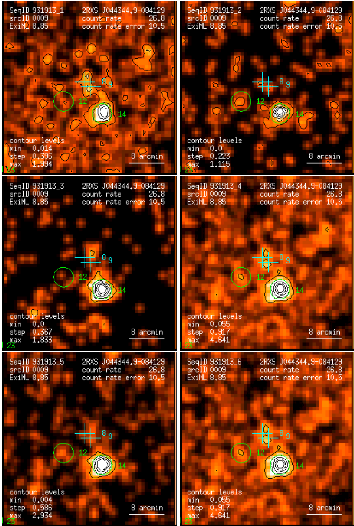
Figure 9: RASS 931913: detection 0009: band rate images, Gaussian filter: (1) PSPC channels 11 – 41, (2) 52 – 90, (3) 91 – 201, (4) 11 – 235, (5) 52 – 201, (6) 11 – 201. Broad band rates in counts/ks. Band rate contour levels in counts/ks/arcmin 2 .
