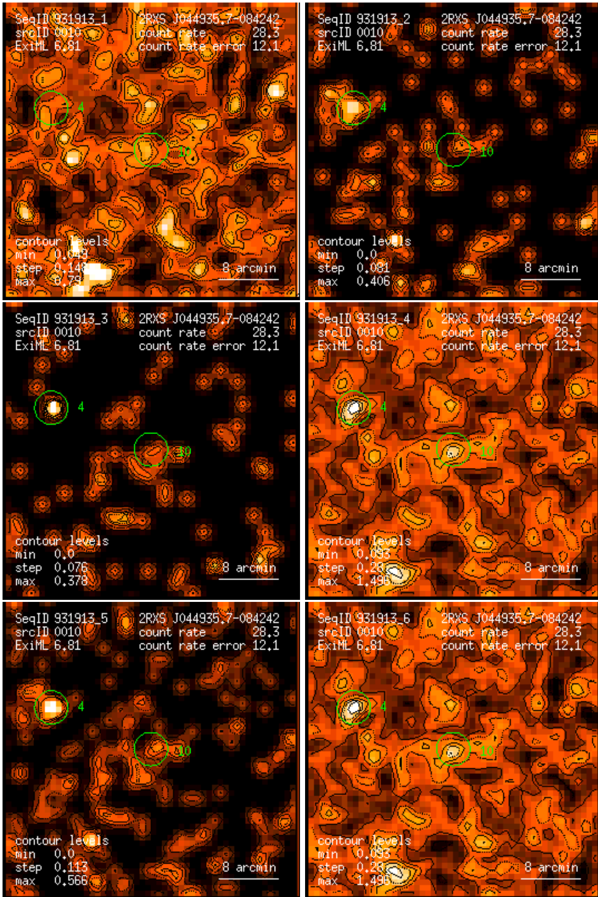
Figure 10: RASS 931913: detection 0010: band rate images, Gaussian filter: (1) PSPC channels 11 – 41, (2) 52 – 90, (3) 91 – 201, (4) 11 – 235, (5) 52 – 201, (6) 11 – 201. Broad band rates in counts/ks. Band rate contour levels in counts/ks/arcmin 2 .
