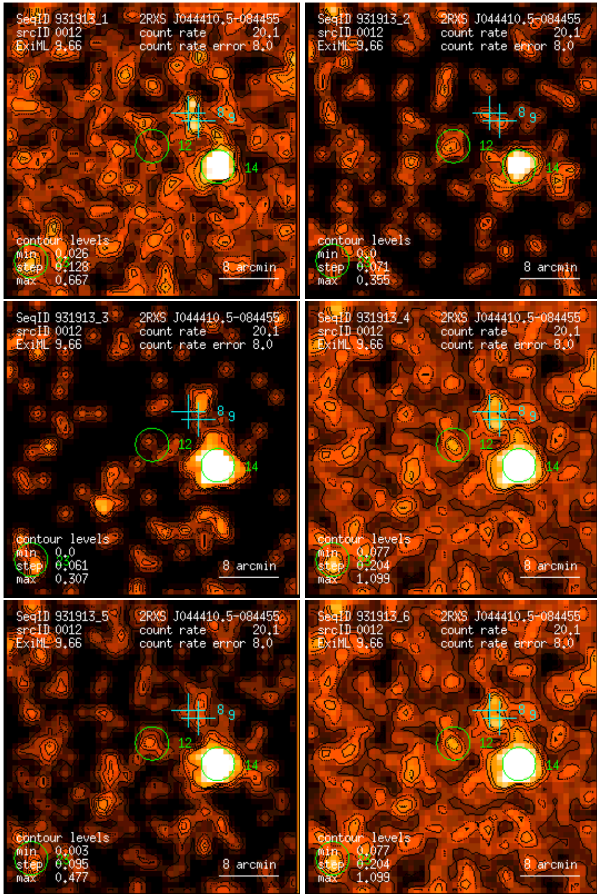
Figure 12: RASS 931913: detection 0012: band rate images, Gaussian filter: (1) PSPC channels 11 – 41, (2) 52 – 90, (3) 91 – 201, (4) 11 – 235, (5) 52 – 201, (6) 11 – 201. Broad band rates in counts/ks. Band rate contour levels in counts/ks/arcmin 2 .
