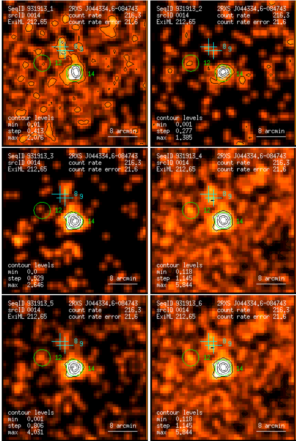
Figure 14: RASS 931913: detection 0014: band rate images, Gaussian filter: (1) PSPC channels 11 – 41, (2) 52 – 90, (3) 91 – 201, (4) 11 – 235, (5) 52 – 201, (6) 11 – 201. Broad band rates in counts/ks. Band rate contour levels in counts/ks/arcmin 2 .
