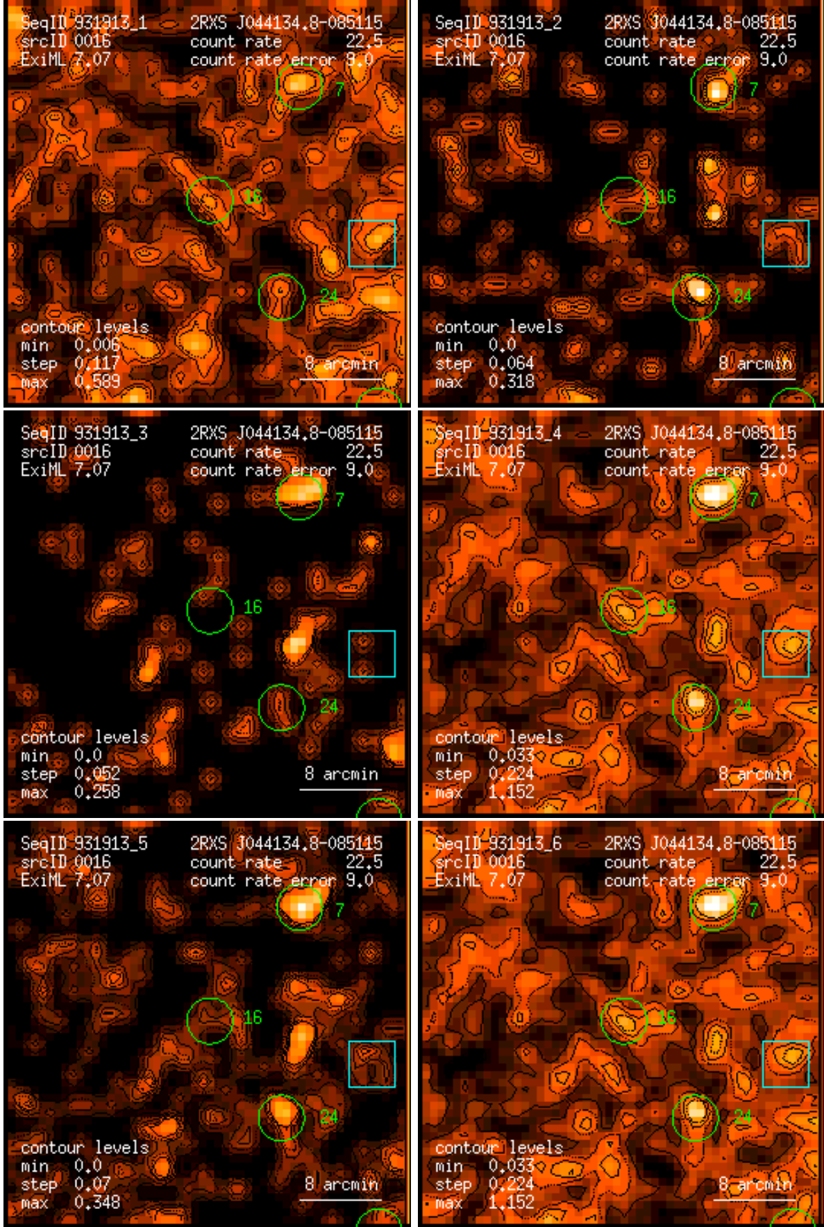
Figure 16: RASS 931913: detection 0016: band rate images, Gaussian filter: (1) PSPC channels 11 – 41, (2) 52 – 90, (3) 91 – 201, (4) 11 – 235, (5) 52 – 201, (6) 11 – 201. Broad band rates in counts/ks. Band rate contour levels in counts/ks/arcmin 2 .
