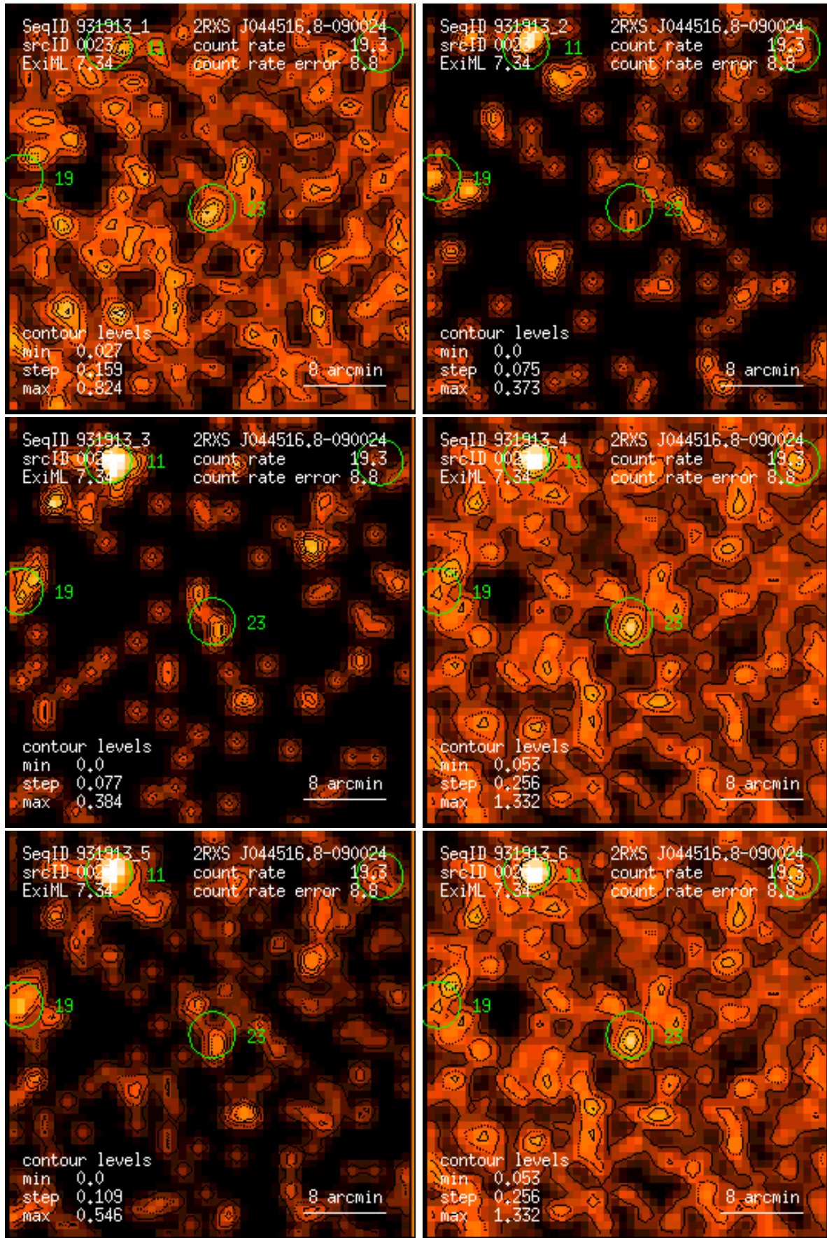
Figure 23: RASS 931913: detection 0023: band rate images, Gaussian filter: (1) PSPC channels 11 – 41, (2) 52 – 90, (3) 91 – 201, (4) 11 – 235, (5) 52 – 201, (6) 11 – 201. Broad band rates in counts/ks. Band rate contour levels in counts/ks/arcmin 2 .
