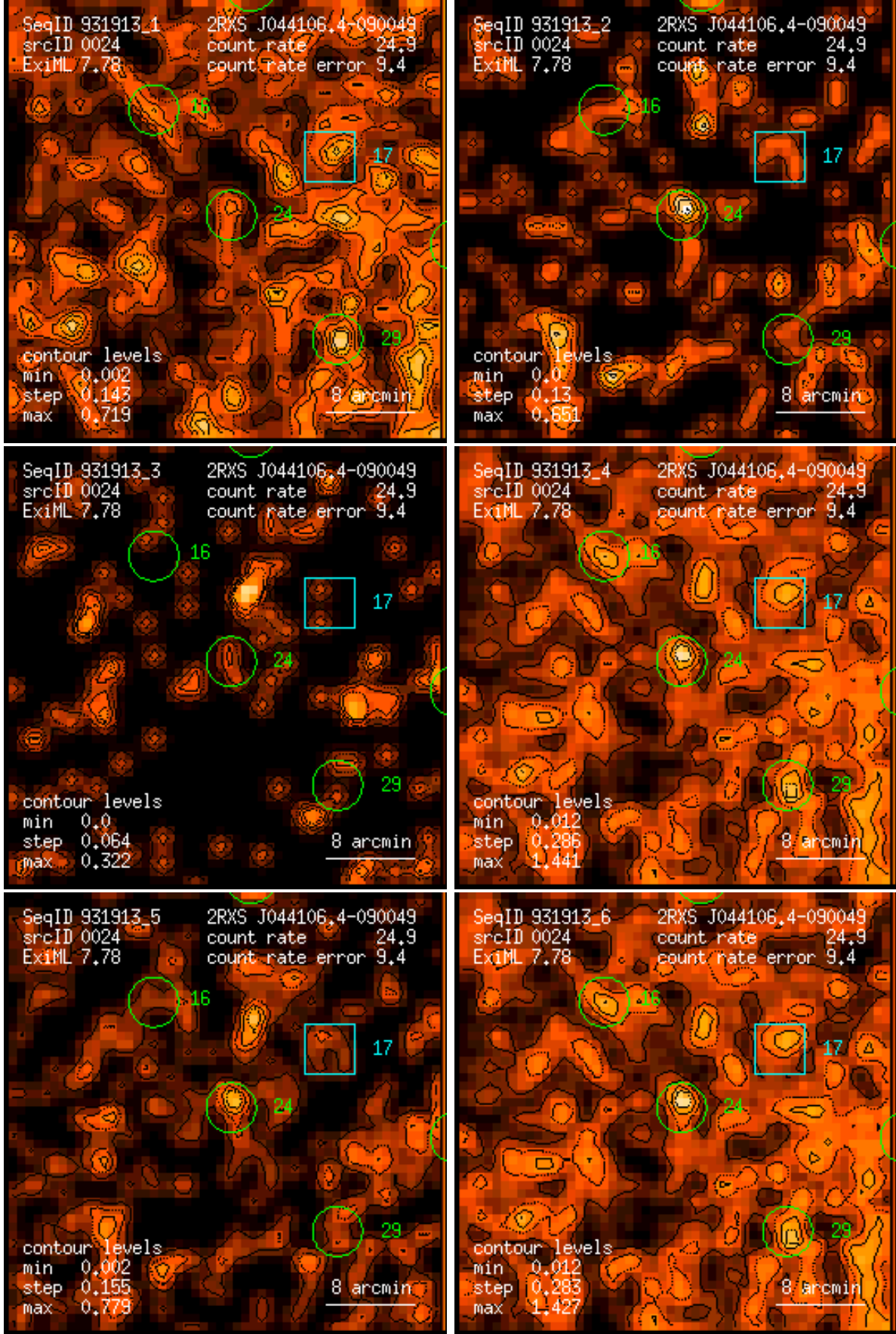
Figure 24: RASS 931913: detection 0024: band rate images, Gaussian filter: (1) PSPC channels 11 – 41, (2) 52 – 90, (3) 91 – 201, (4) 11 – 235, (5) 52 – 201, (6) 11 – 201. Broad band rates in counts/ks. Band rate contour levels in counts/ks/arcmin 2 .
