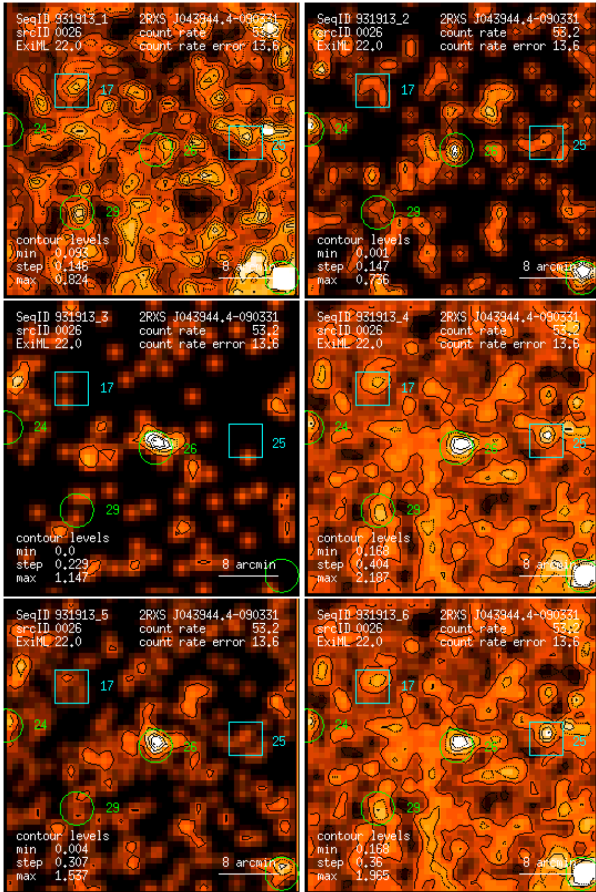
Figure 26: RASS 931913: detection 0026: band rate images, Gaussian filter: (1) PSPC channels 11 – 41, (2) 52 – 90, (3) 91 – 201, (4) 11 – 235, (5) 52 – 201, (6) 11 – 201. Broad band rates in counts/ks. Band rate contour levels in counts/ks/arcmin 2 .
