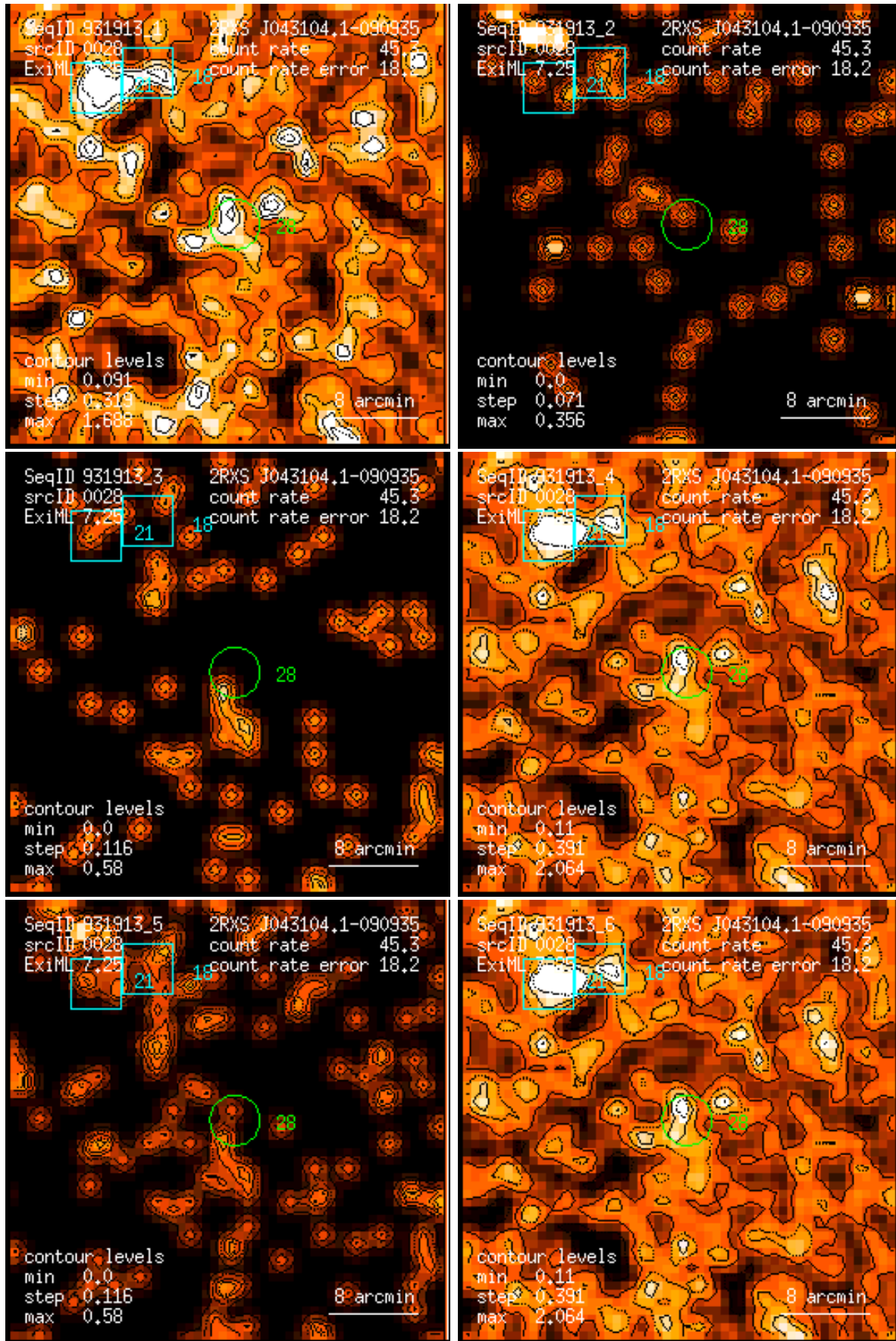
Figure 28: RASS 931913: detection 0028: band rate images, Gaussian filter: (1) PSPC channels 11 – 41, (2) 52 – 90, (3) 91 – 201, (4) 11 – 235, (5) 52 – 201, (6) 11 – 201. Broad band rates in counts/ks. Band rate contour levels in counts/ks/arcmin 2 .
