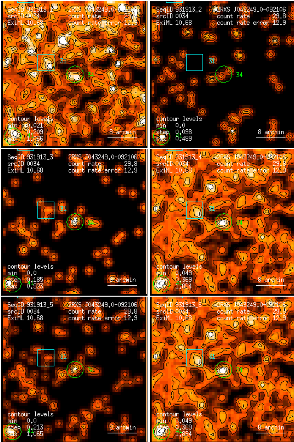
Figure 34: RASS 931913: detection 0034: band rate images, Gaussian filter: (1) PSPC channels 11 – 41, (2) 52 – 90, (3) 91 – 201, (4) 11 – 235, (5) 52 – 201, (6) 11 – 201. Broad band rates in counts/ks. Band rate contour levels in counts/ks/arcmin 2 .
