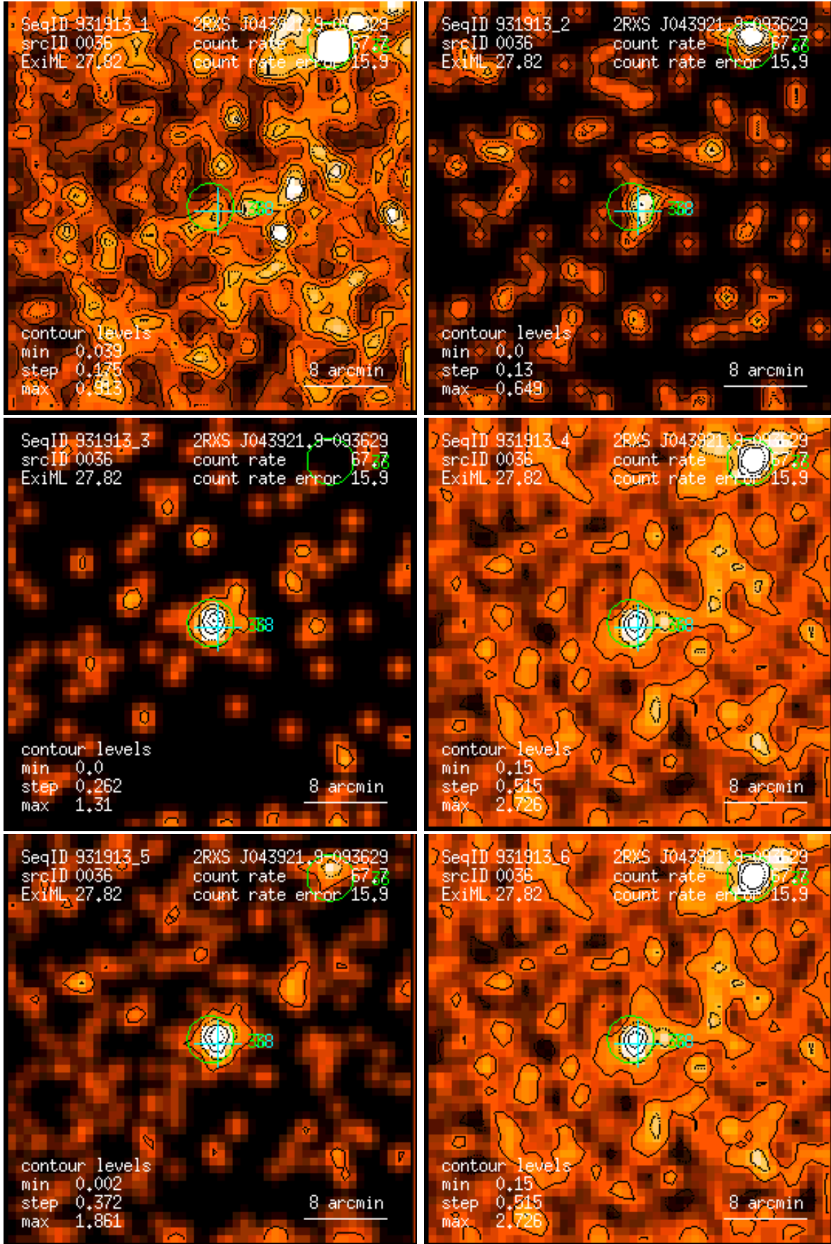
Figure 36: RASS 931913: detection 0036: band rate images, Gaussian filter: (1) PSPC channels 11 – 41, (2) 52 – 90, (3) 91 – 201, (4) 11 – 235, (5) 52 – 201, (6) 11 – 201. Broad band rates in counts/ks. Band rate contour levels in counts/ks/arcmin 2 .
