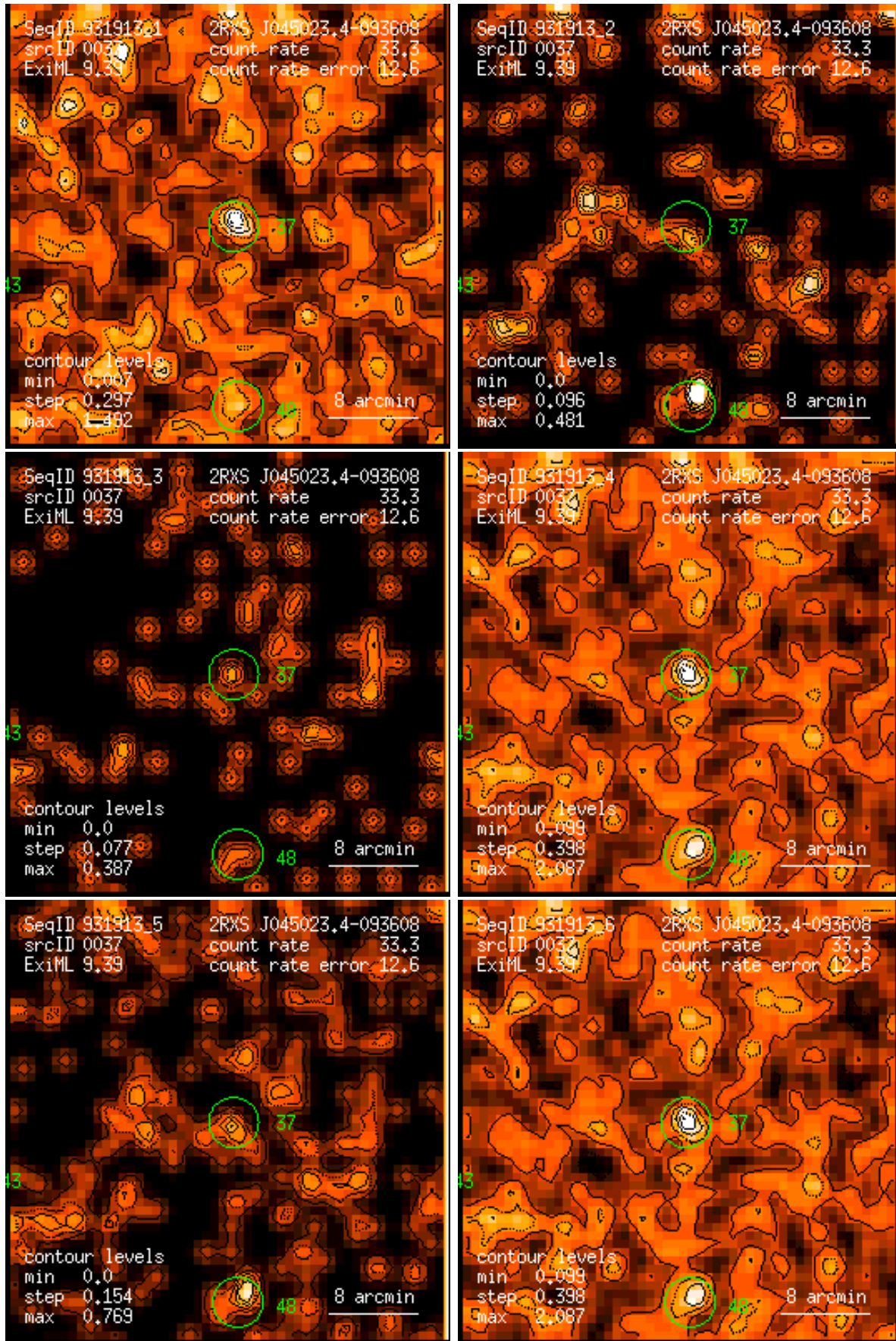
Figure 37: RASS 931913: detection 0037: band rate images, Gaussian filter: (1) PSPC channels 11 – 41, (2) 52 – 90, (3) 91 – 201, (4) 11 – 235, (5) 52 – 201, (6) 11 – 201. Broad band rates in counts/ks. Band rate contour levels in counts/ks/arcmin 2 .
