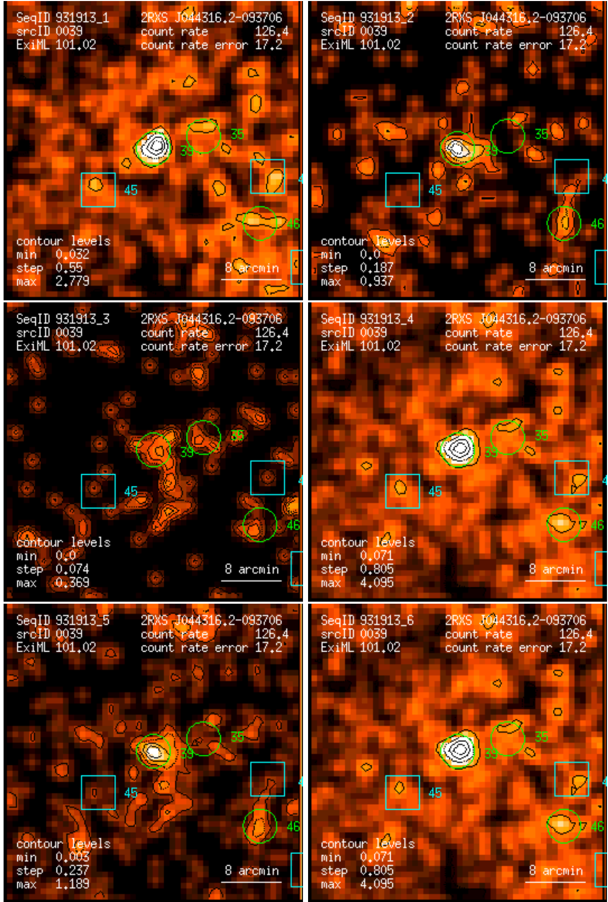
Figure 39: RASS 931913: detection 0039: band rate images, Gaussian filter: (1) PSPC channels 11 – 41, (2) 52 – 90, (3) 91 – 201, (4) 11 – 235, (5) 52 – 201, (6) 11 – 201. Broad band rates in counts/ks. Band rate contour levels in counts/ks/arcmin 2 .
