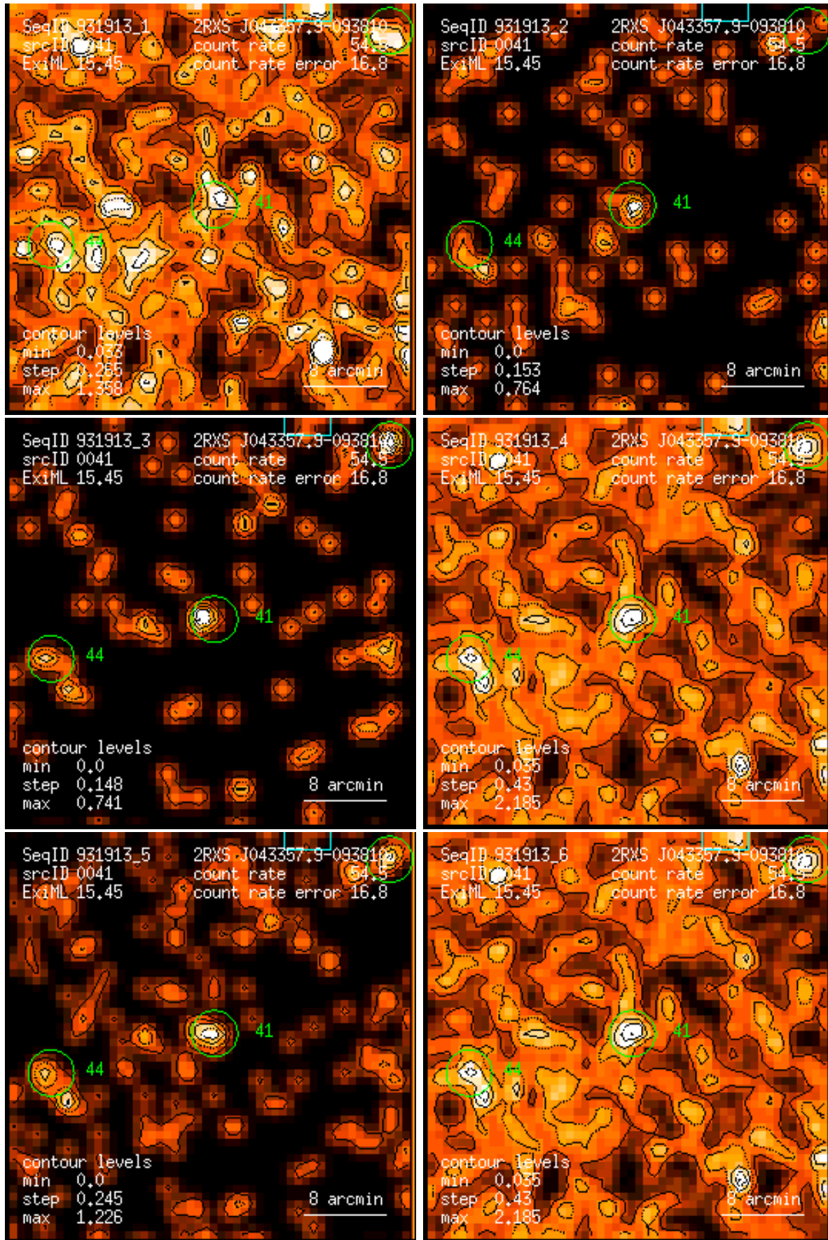
Figure 41: RASS 931913: detection 0041: band rate images, Gaussian filter: (1) PSPC channels 11 – 41, (2) 52 – 90, (3) 91 – 201, (4) 11 – 235, (5) 52 – 201, (6) 11 – 201. Broad band rates in counts/ks. Band rate contour levels in counts/ks/arcmin 2 .
